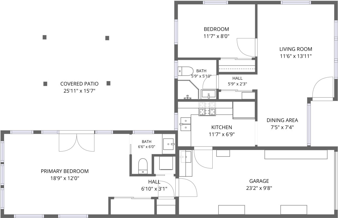
1st floor
