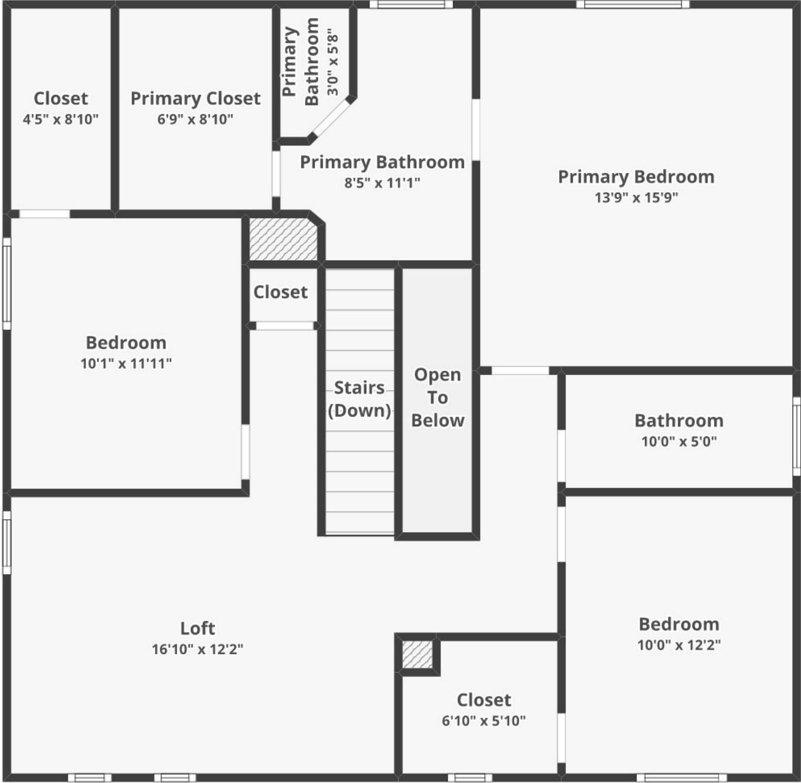
FLOOR 2
