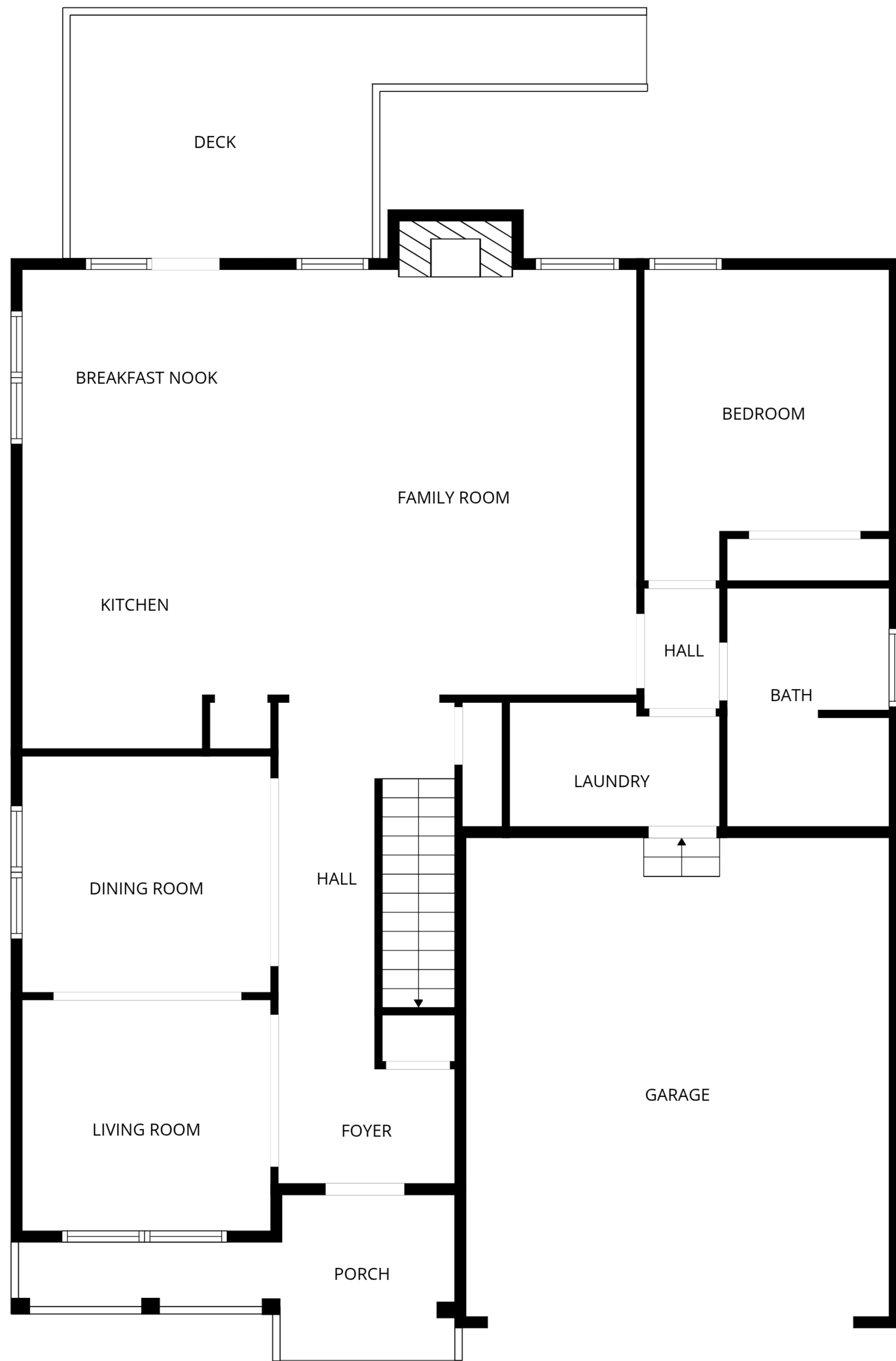
1st floor
