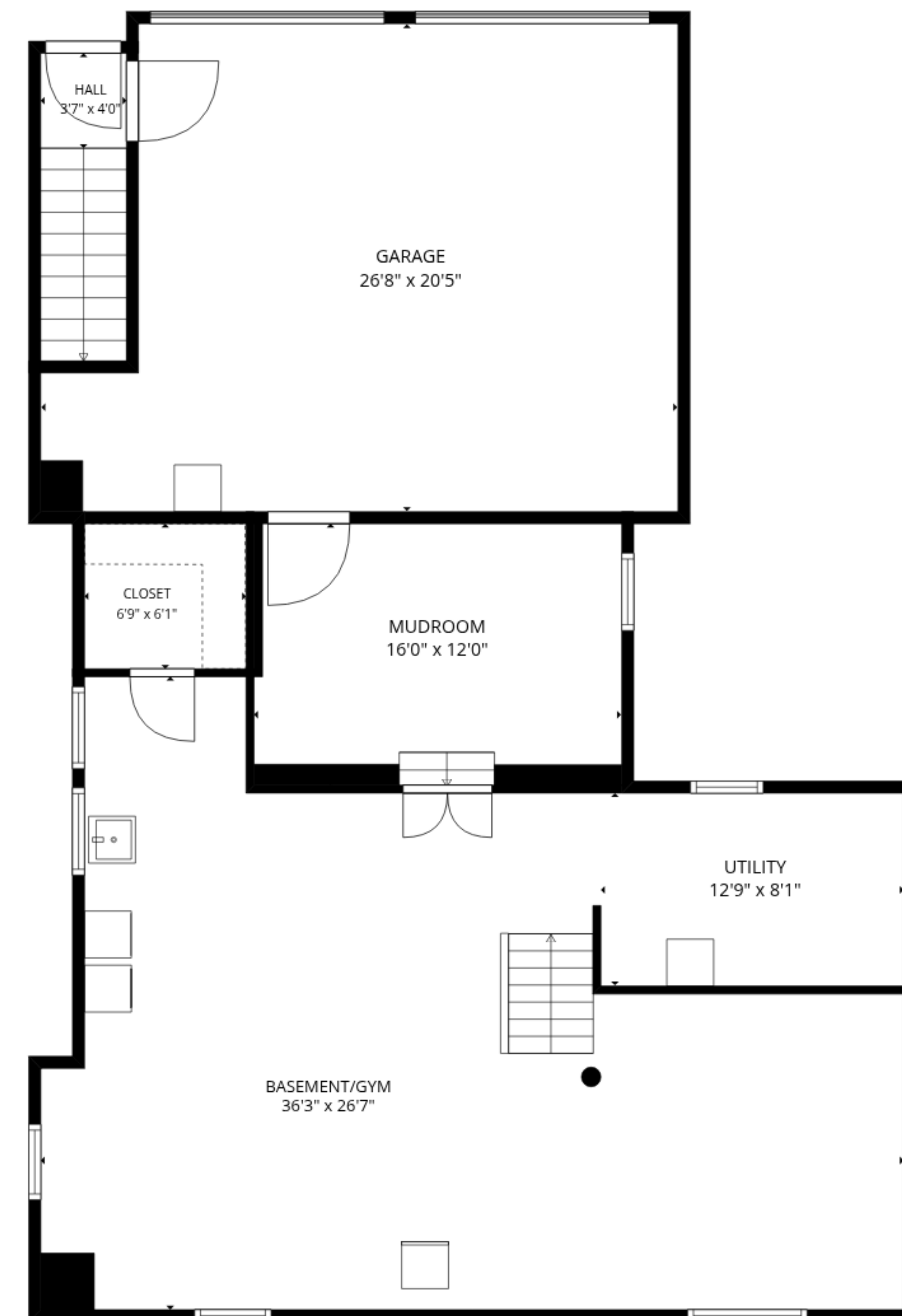
1ST FLOOR
