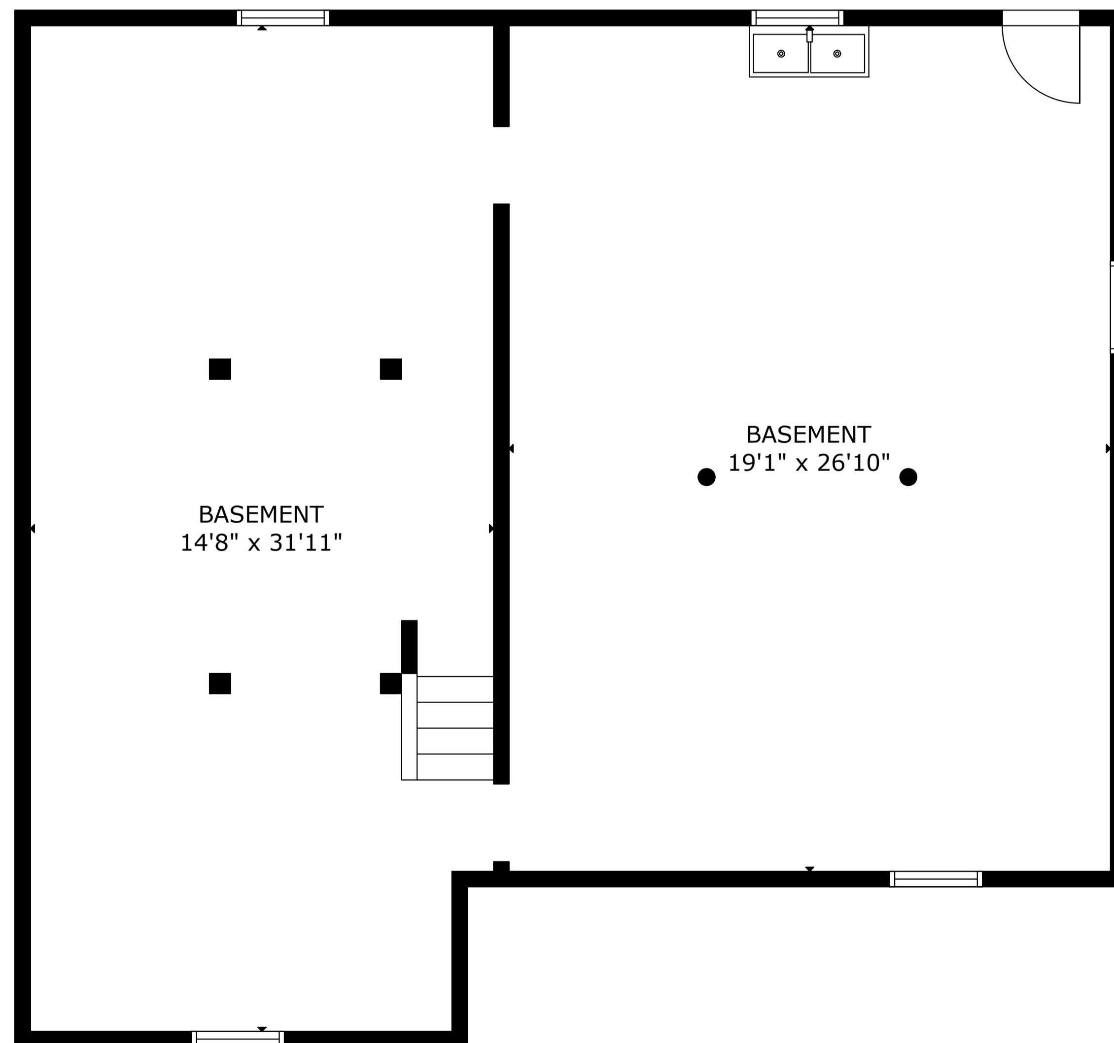
LOWER FLOOR
