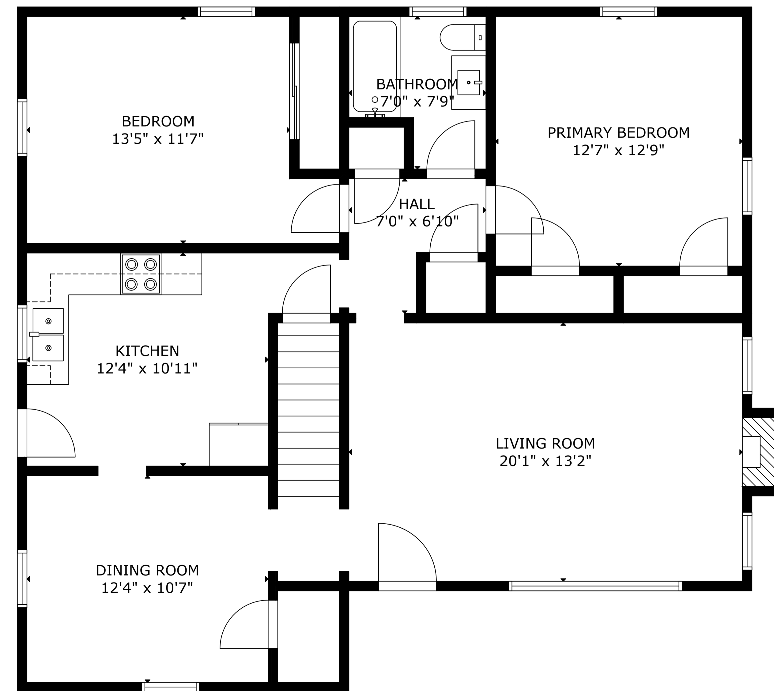
MAIN FLOOR
