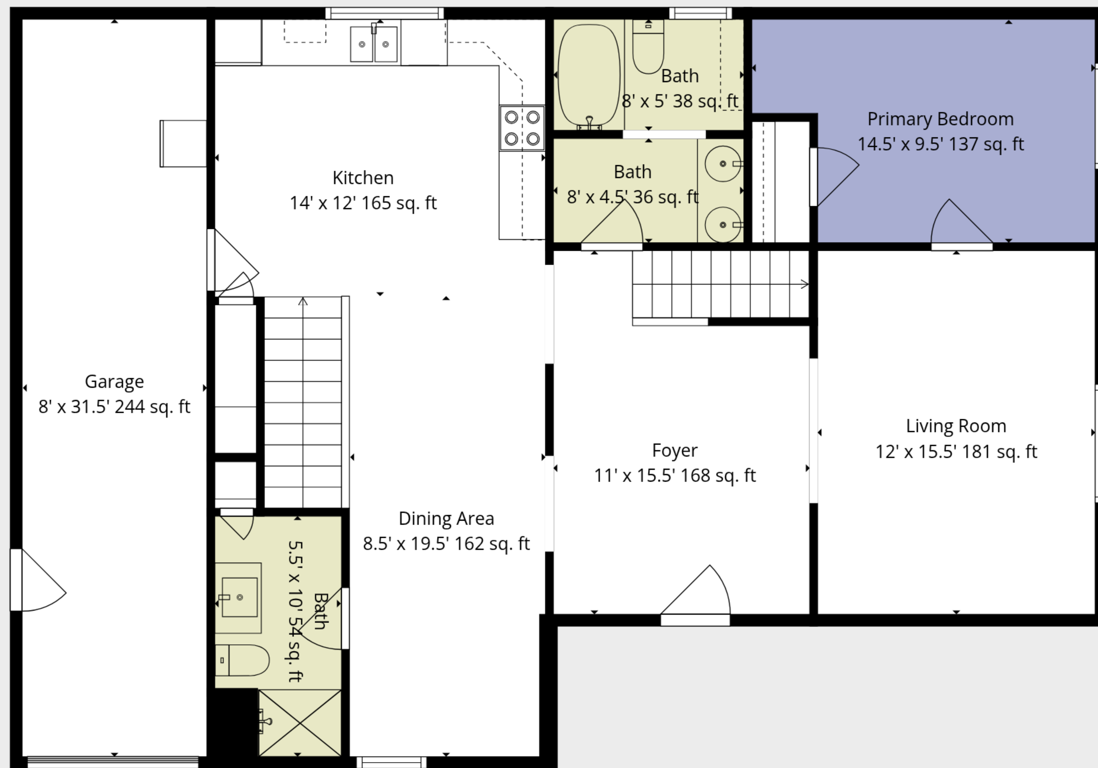
1st Floor
