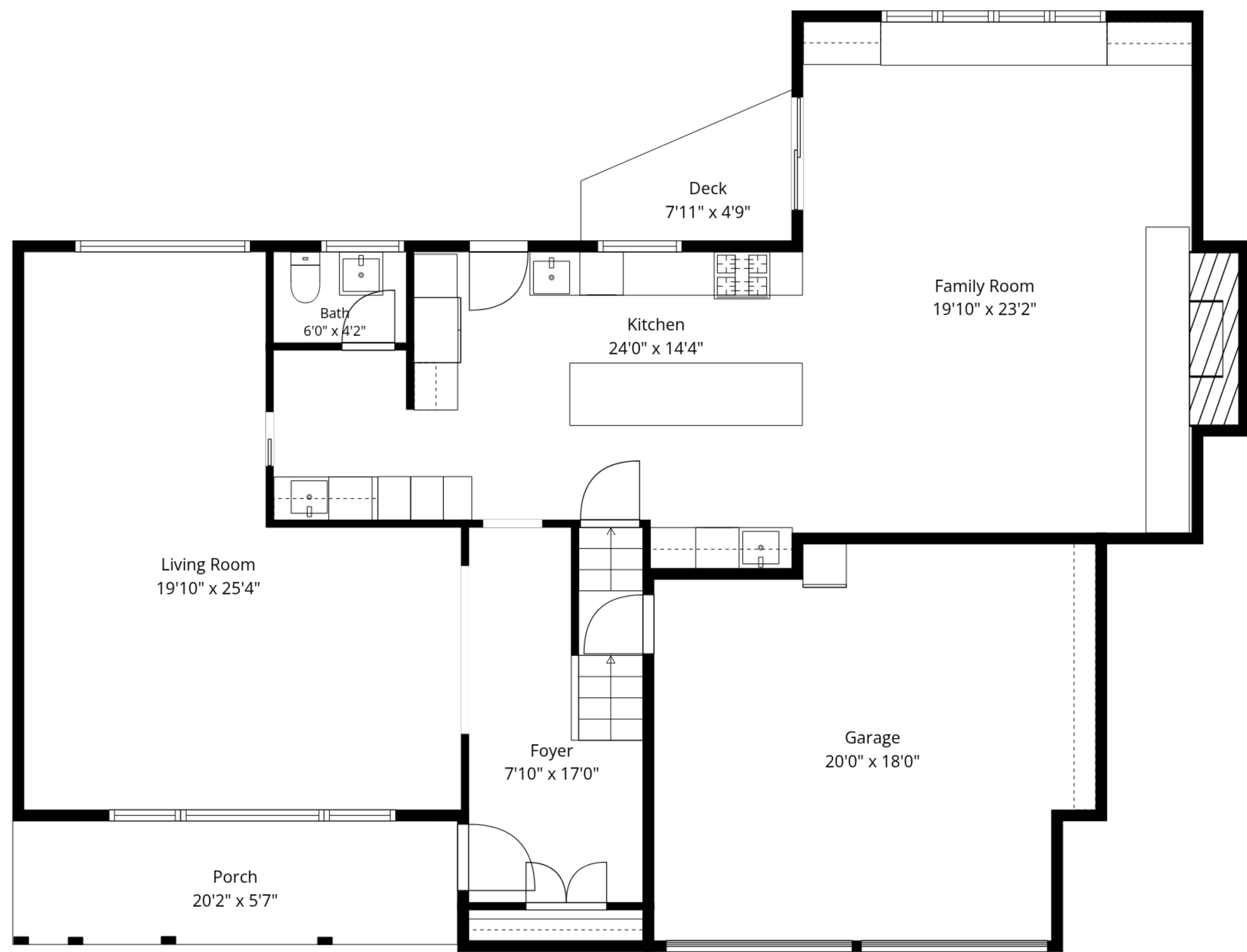
1st Floor
