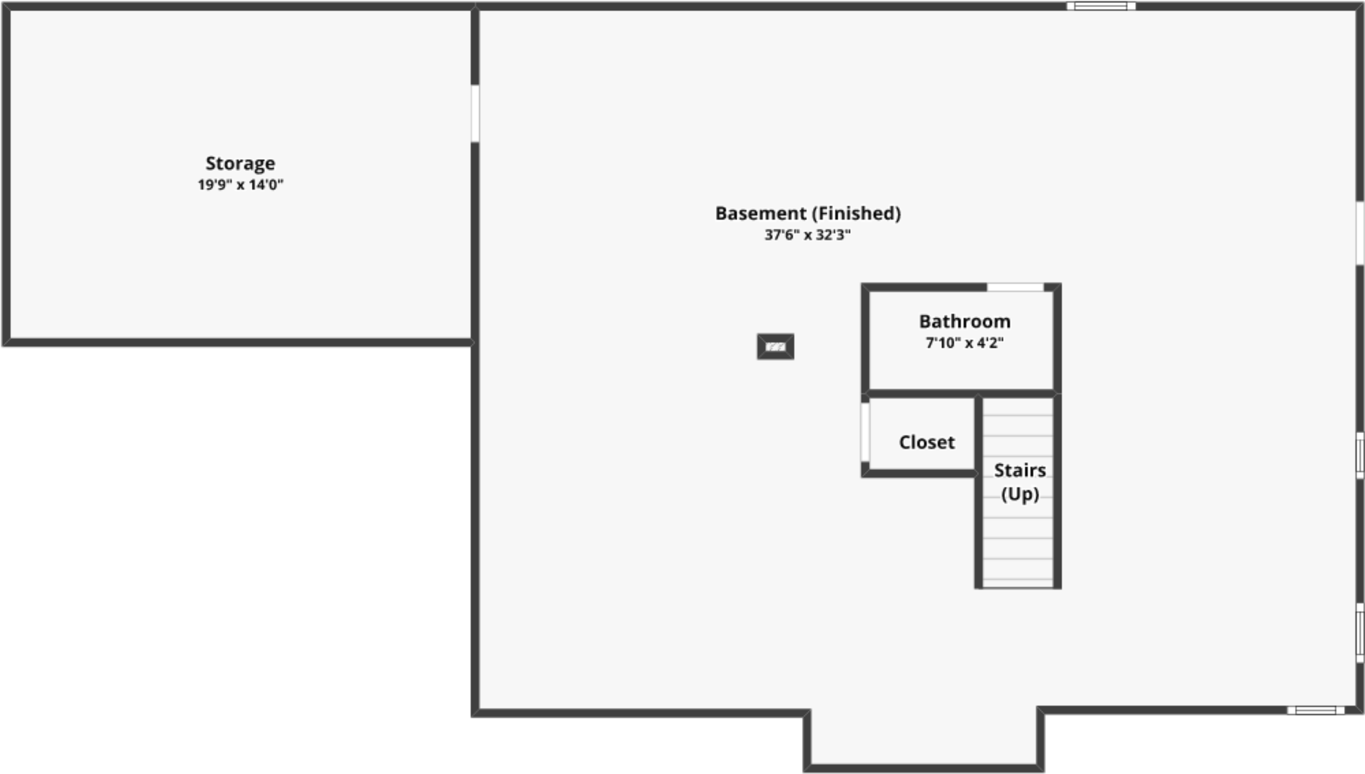
BASEMENT Finished area: ~1,395.66 sq. ft.
