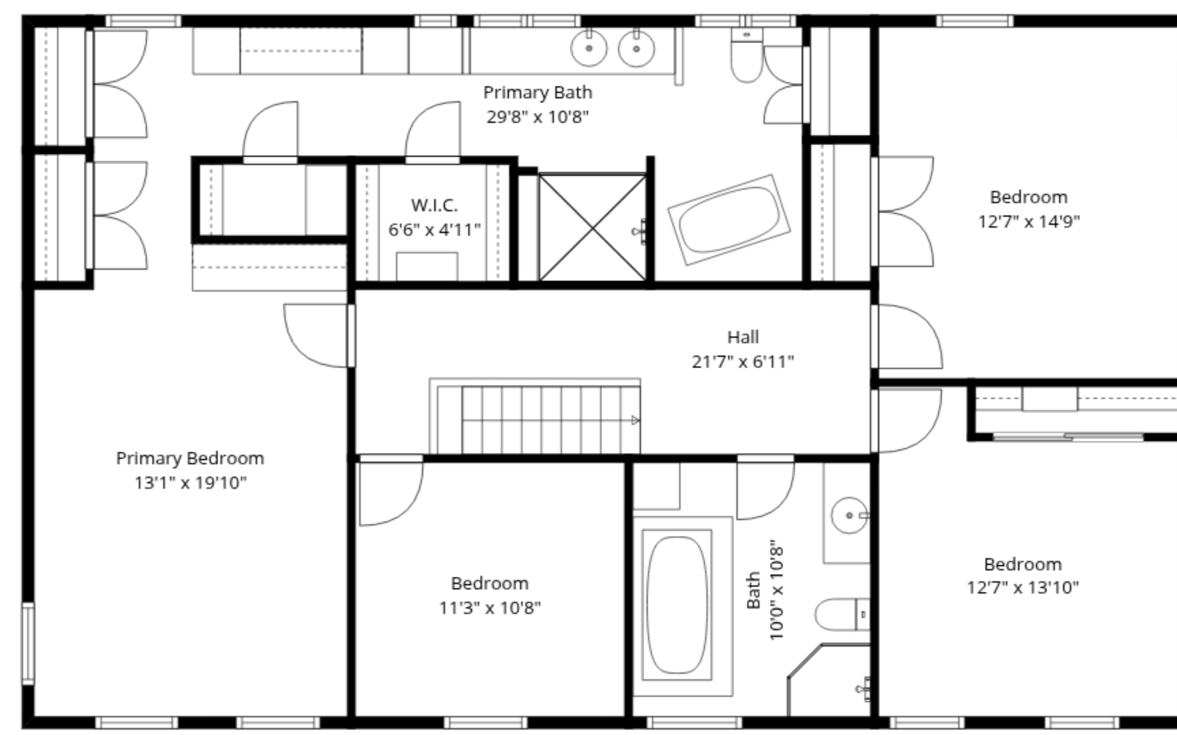
2nd Floor
