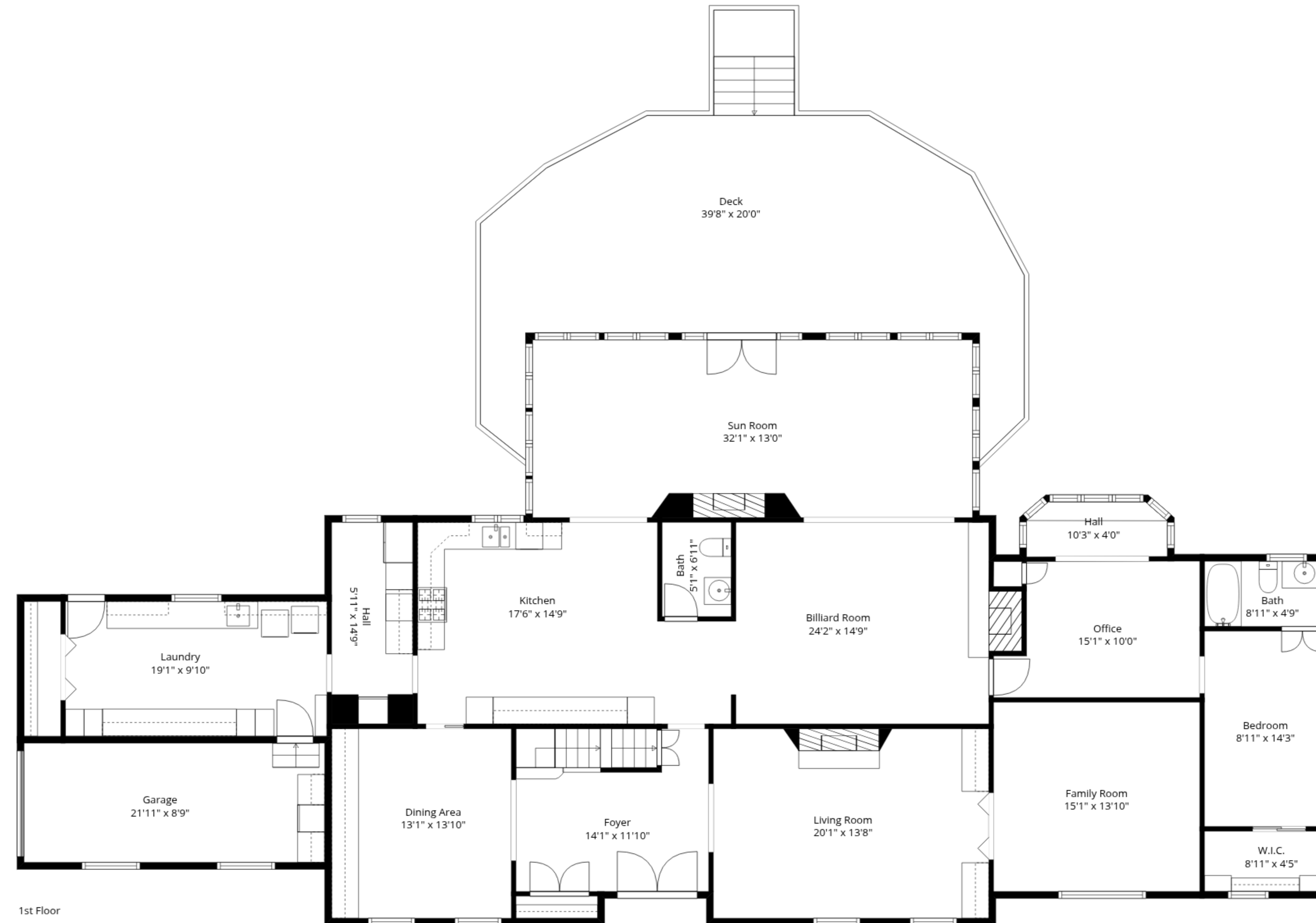
1st Floor
