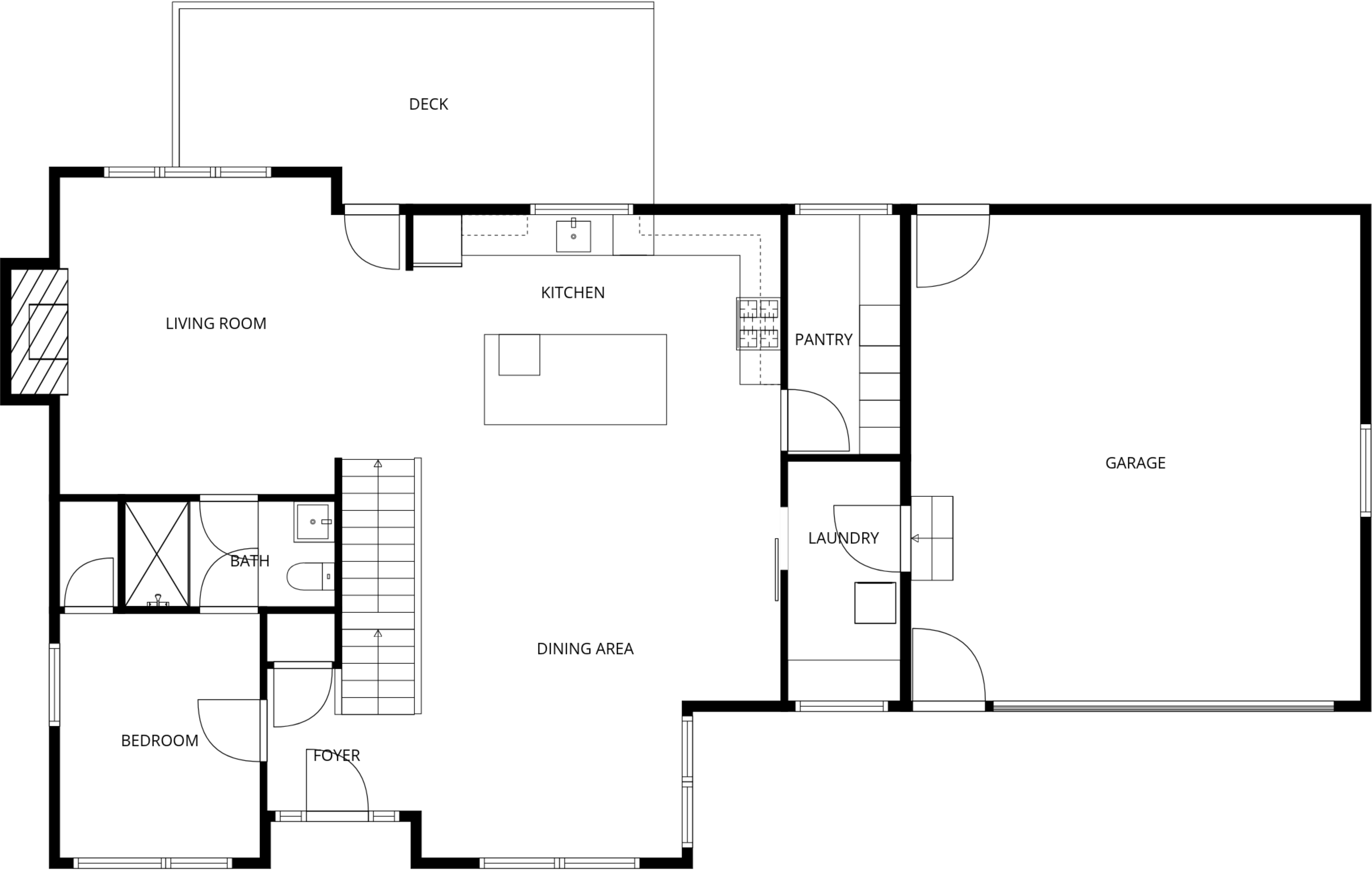
1st floor
