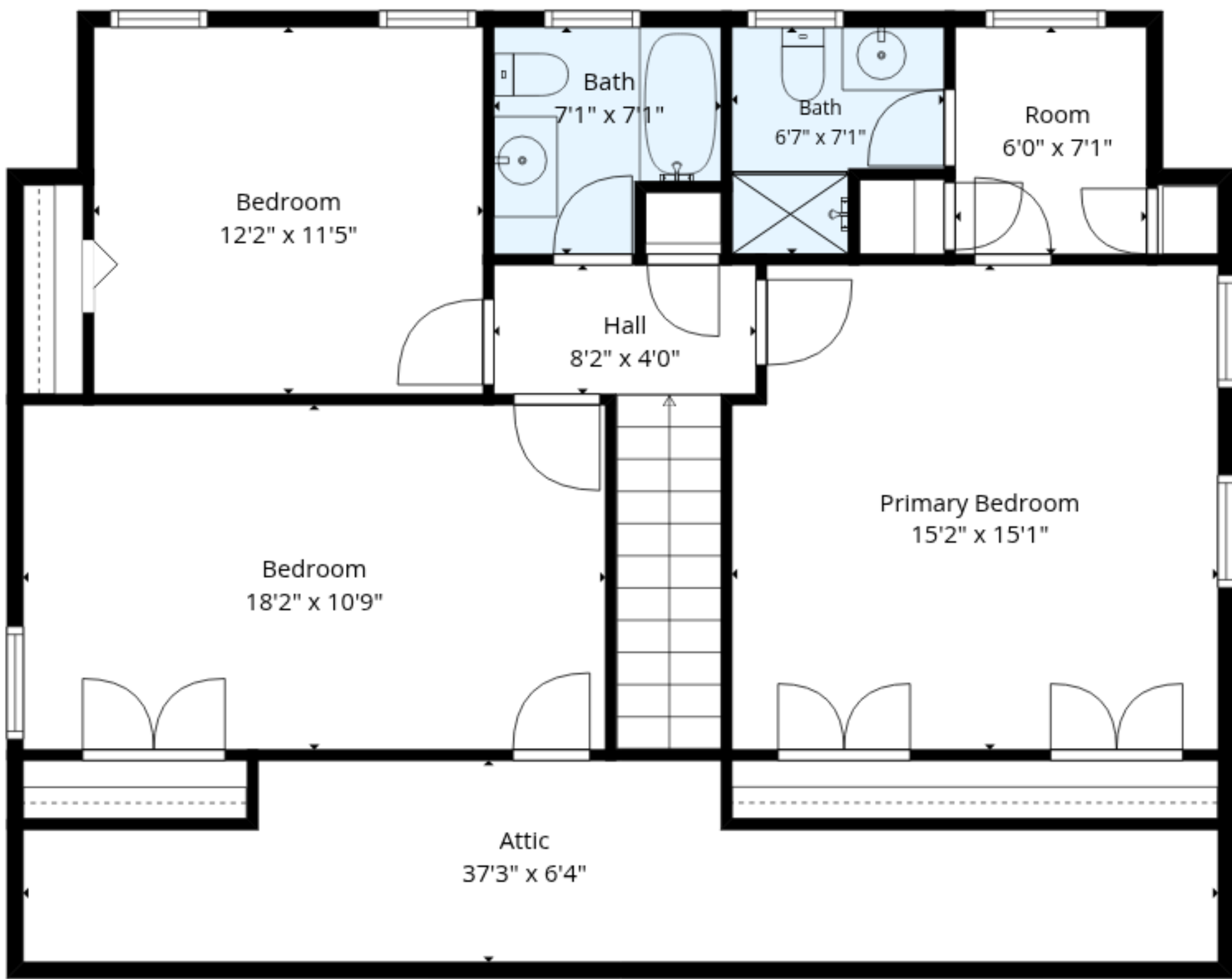
2nd Floor
