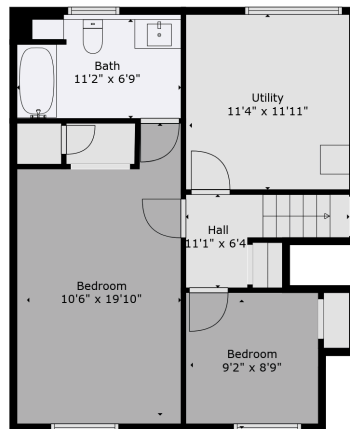
Floor 1
