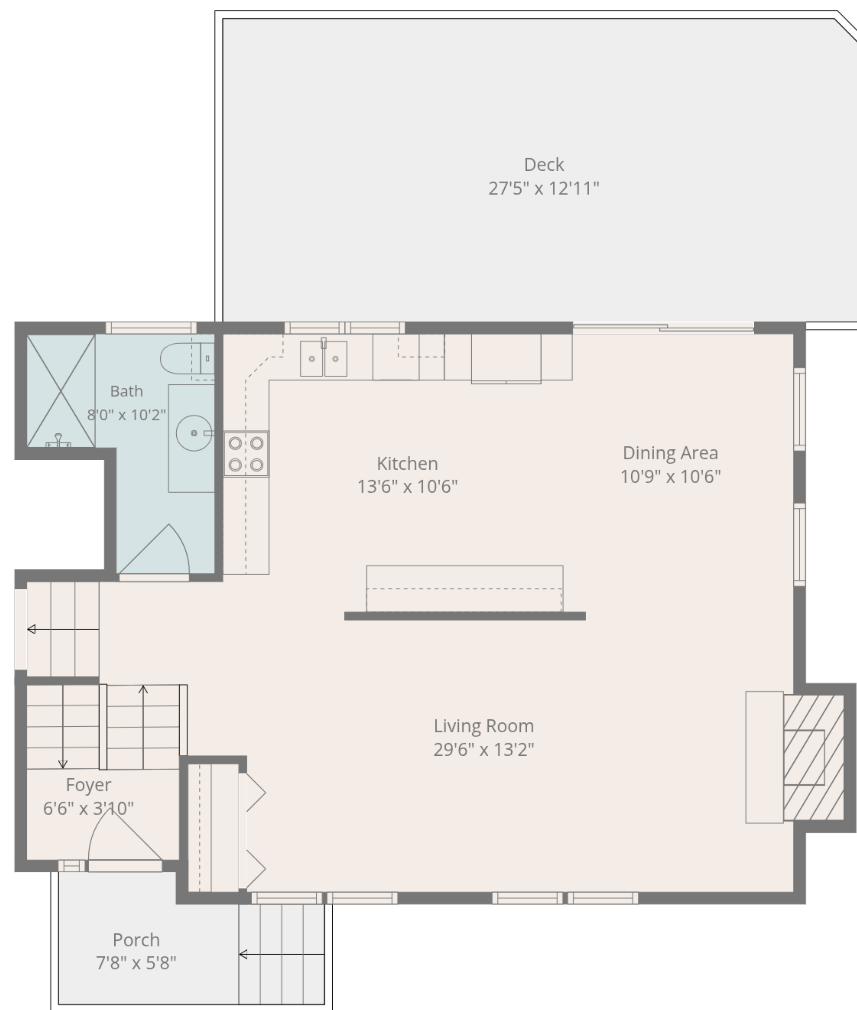
2nd Floor
