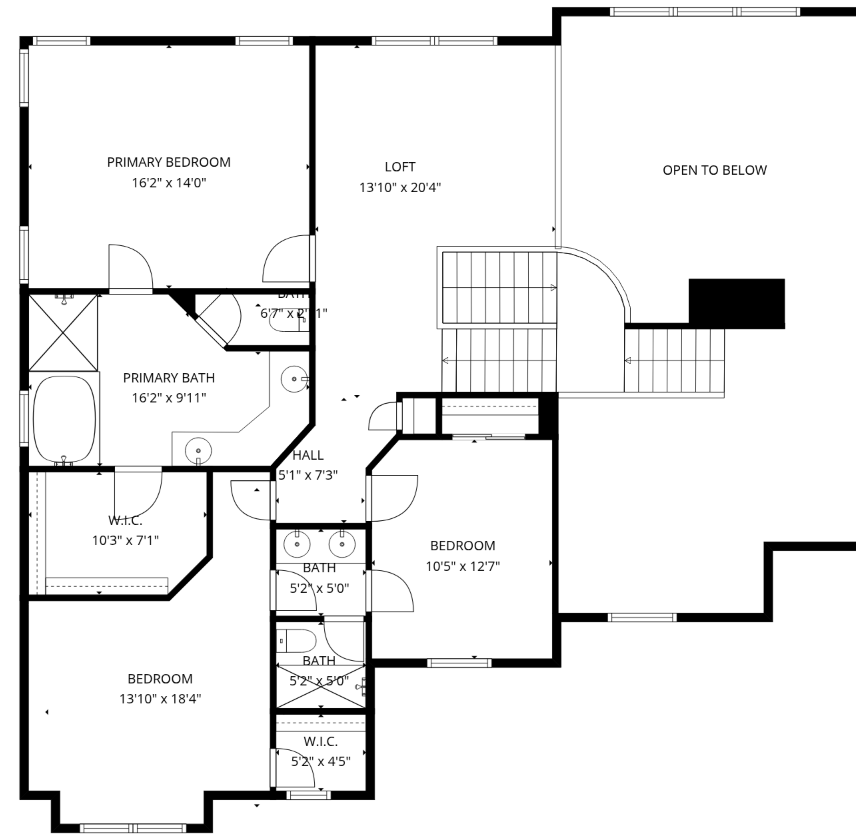
2nd floor
