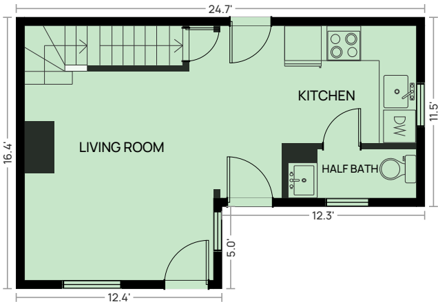
FIRST FLOOR Above grade · 9'0" ceiling · GLA 345 sq ft
