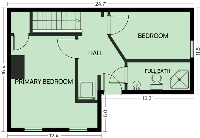
SECOND FLOOR Above grade · 7'1" ceiling · GLA 345 sq ft
