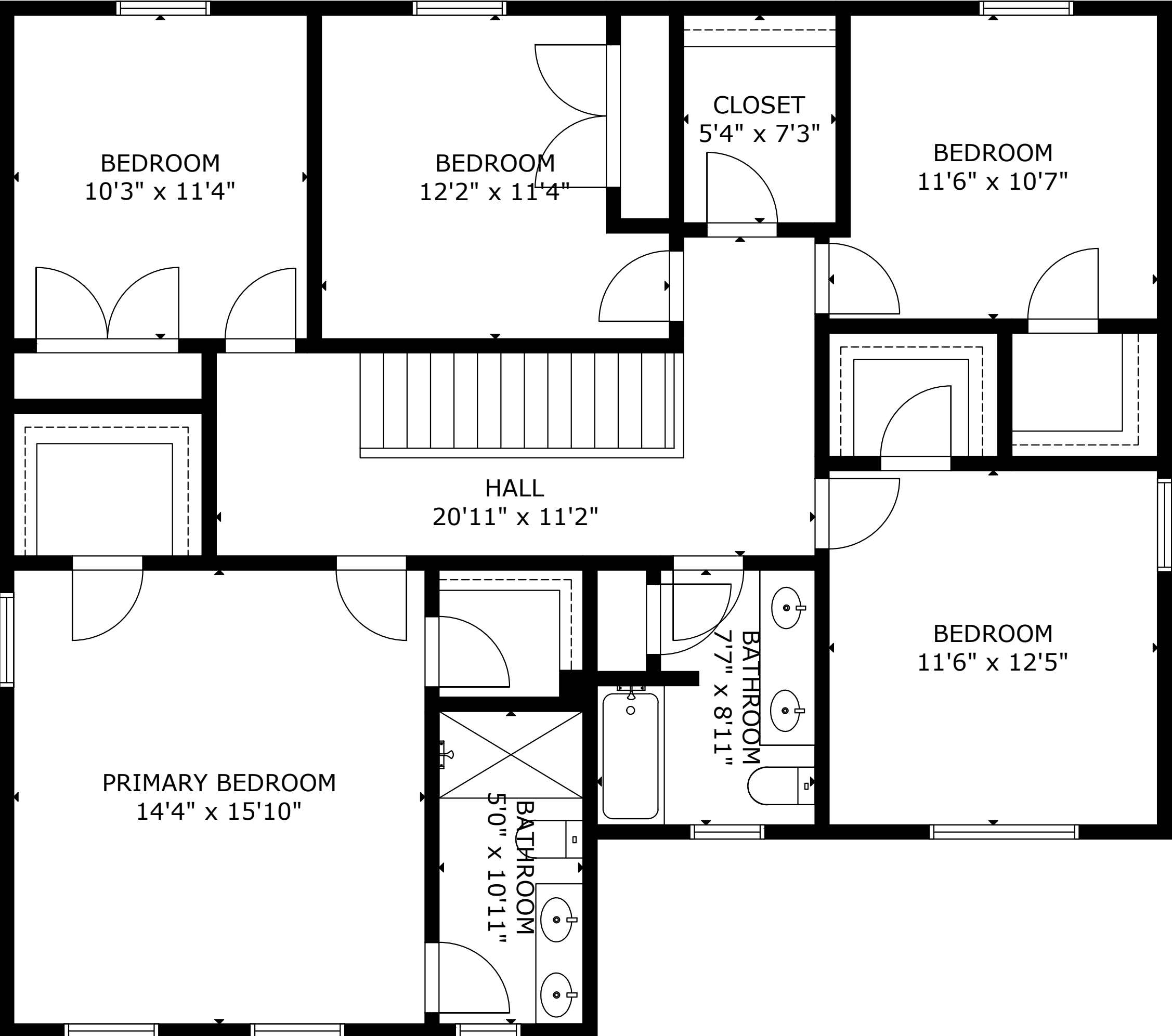
UPPER LEVEL 1
