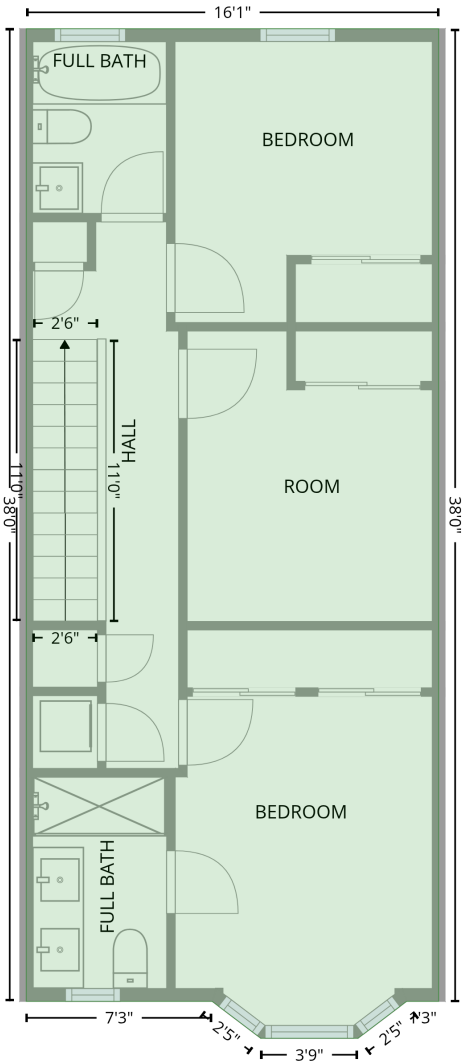
FLOOR 3 [AREA: 619]
