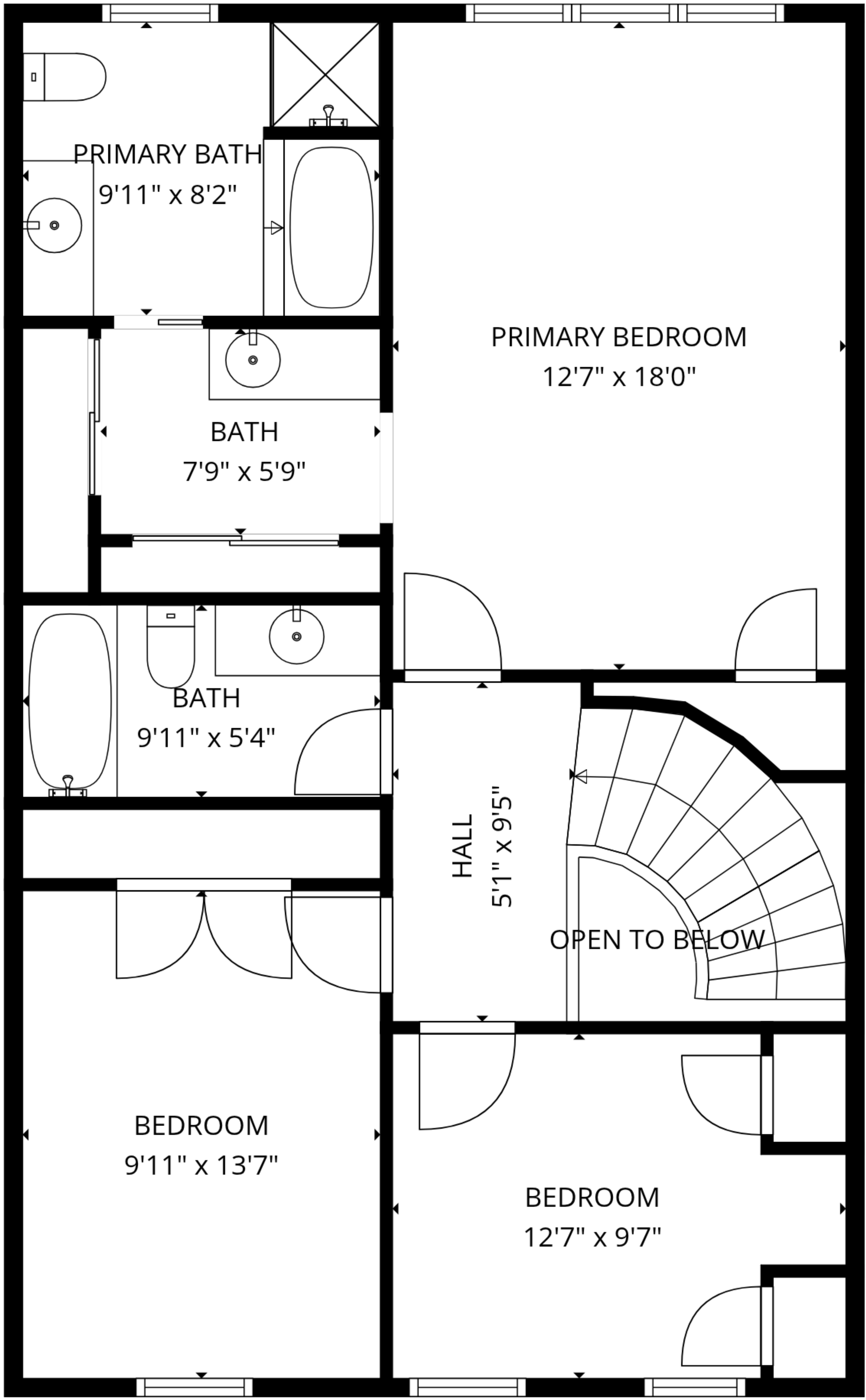
2nd floor
