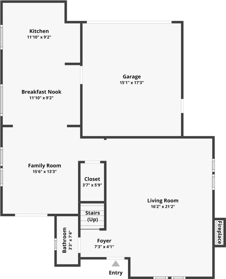
FLOOR 1 Finished area: ~776.85 sq. ft.
