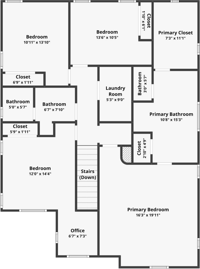
FLOOR 2 Finished area: ~1,234.14 sq. ft.
