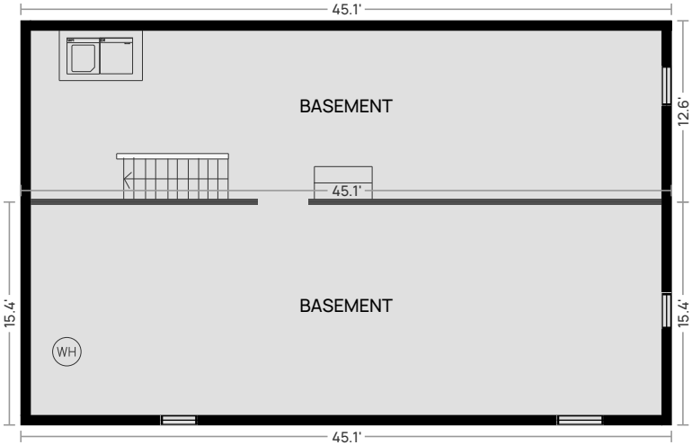
BASEMENT Below grade · 7'10" ceiling · No finished area
