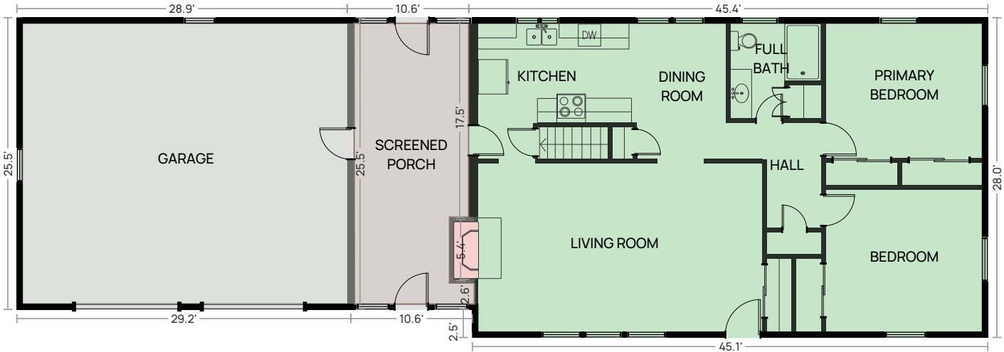
FIRST FLOOR Above grade · 8'0" ceiling · GLA 1,265 sq ft
