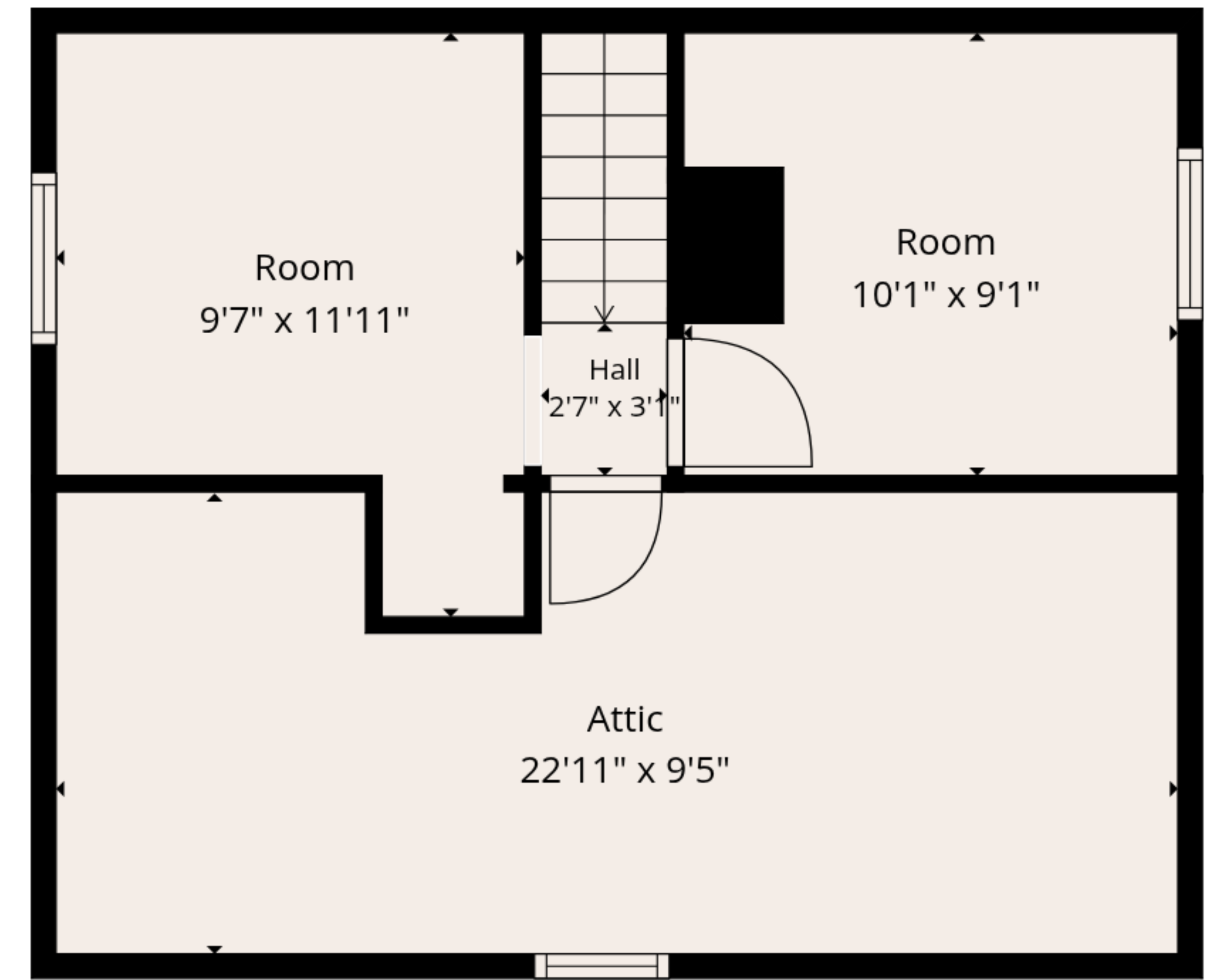
2nd Floor
