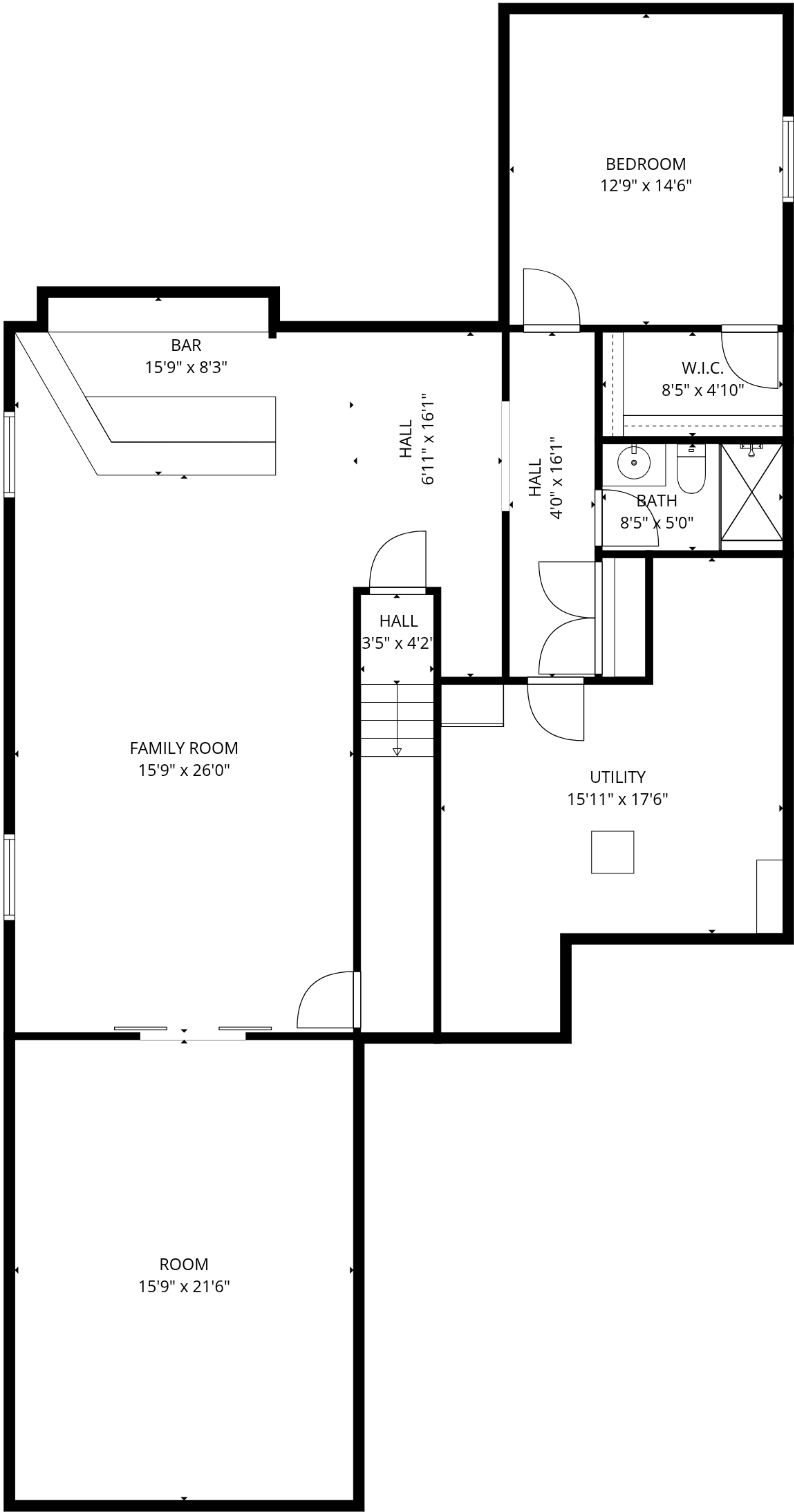
Basement 1
