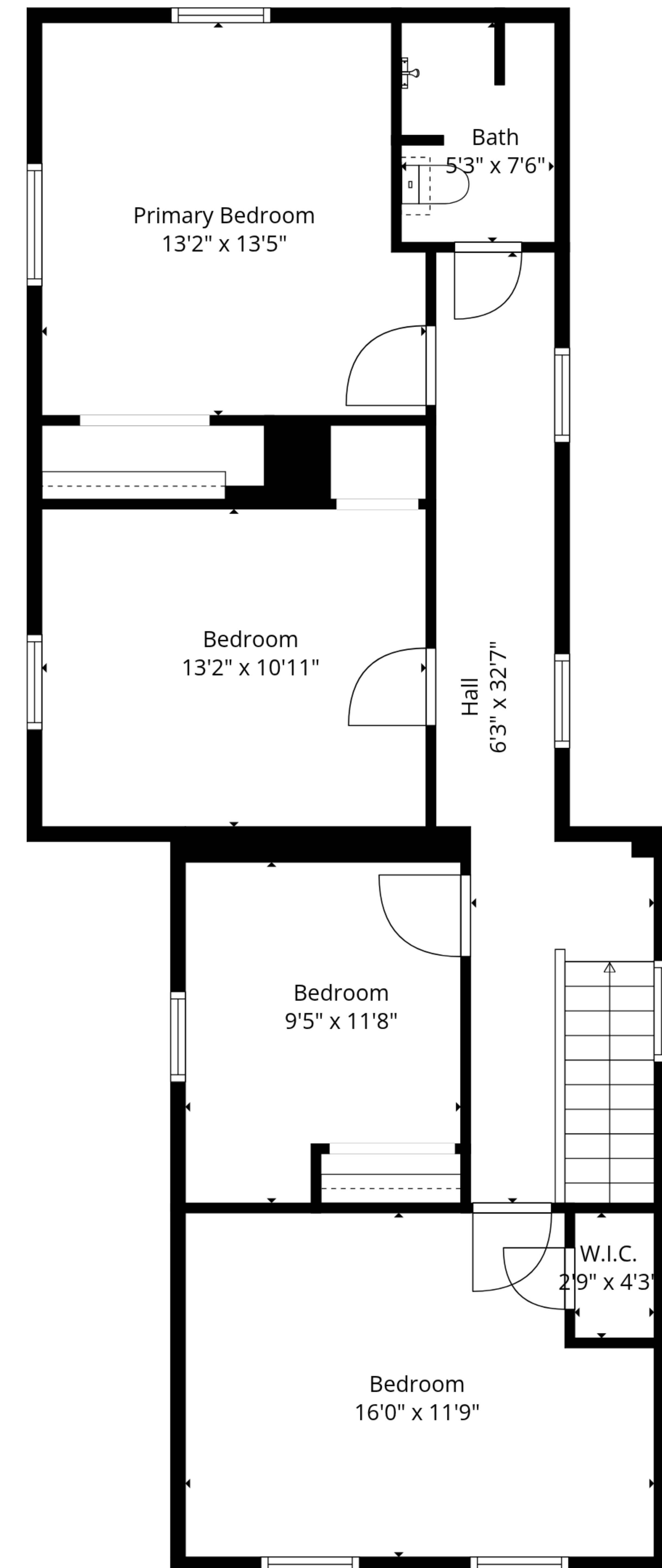
2nd Floor
