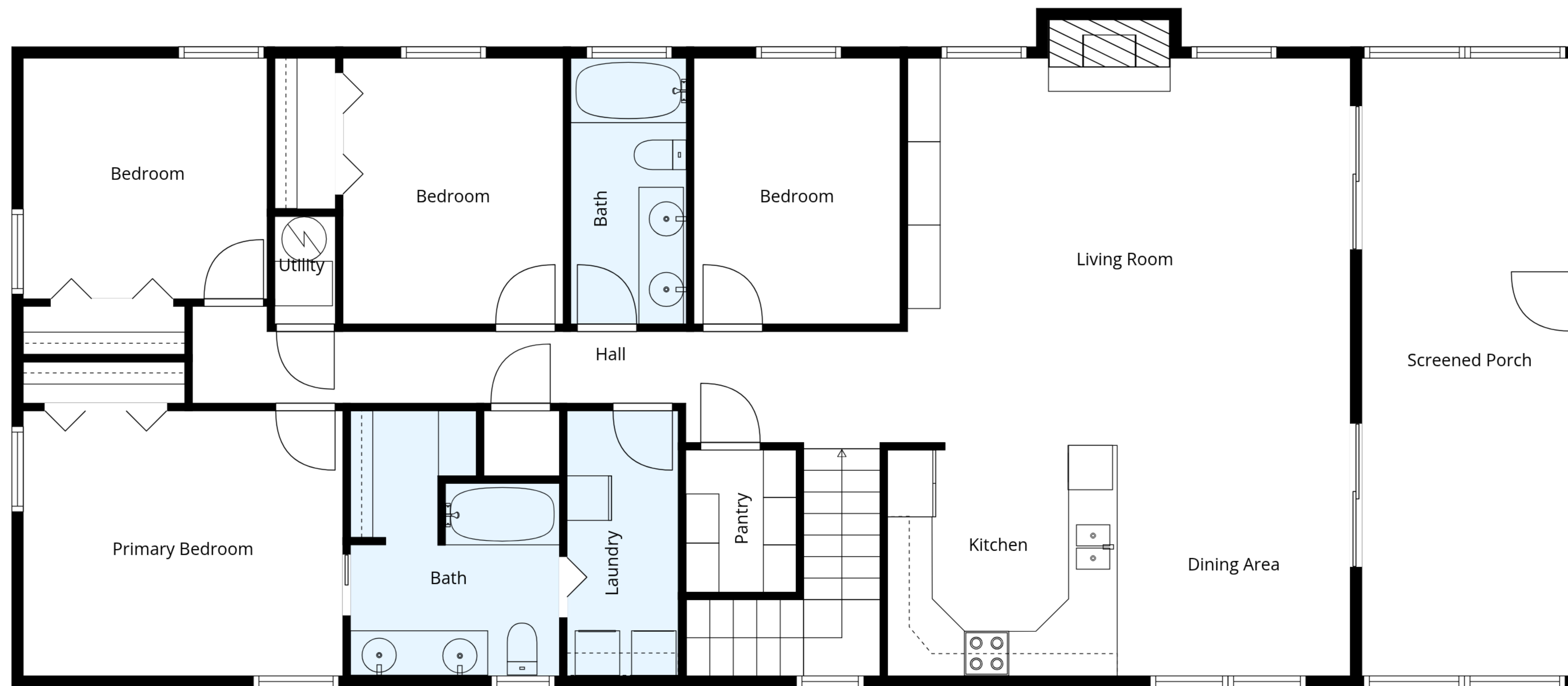
2nd Floor
