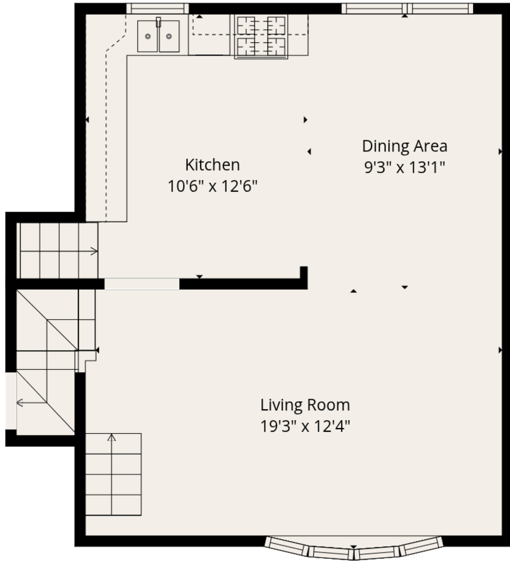
2nd Floor
