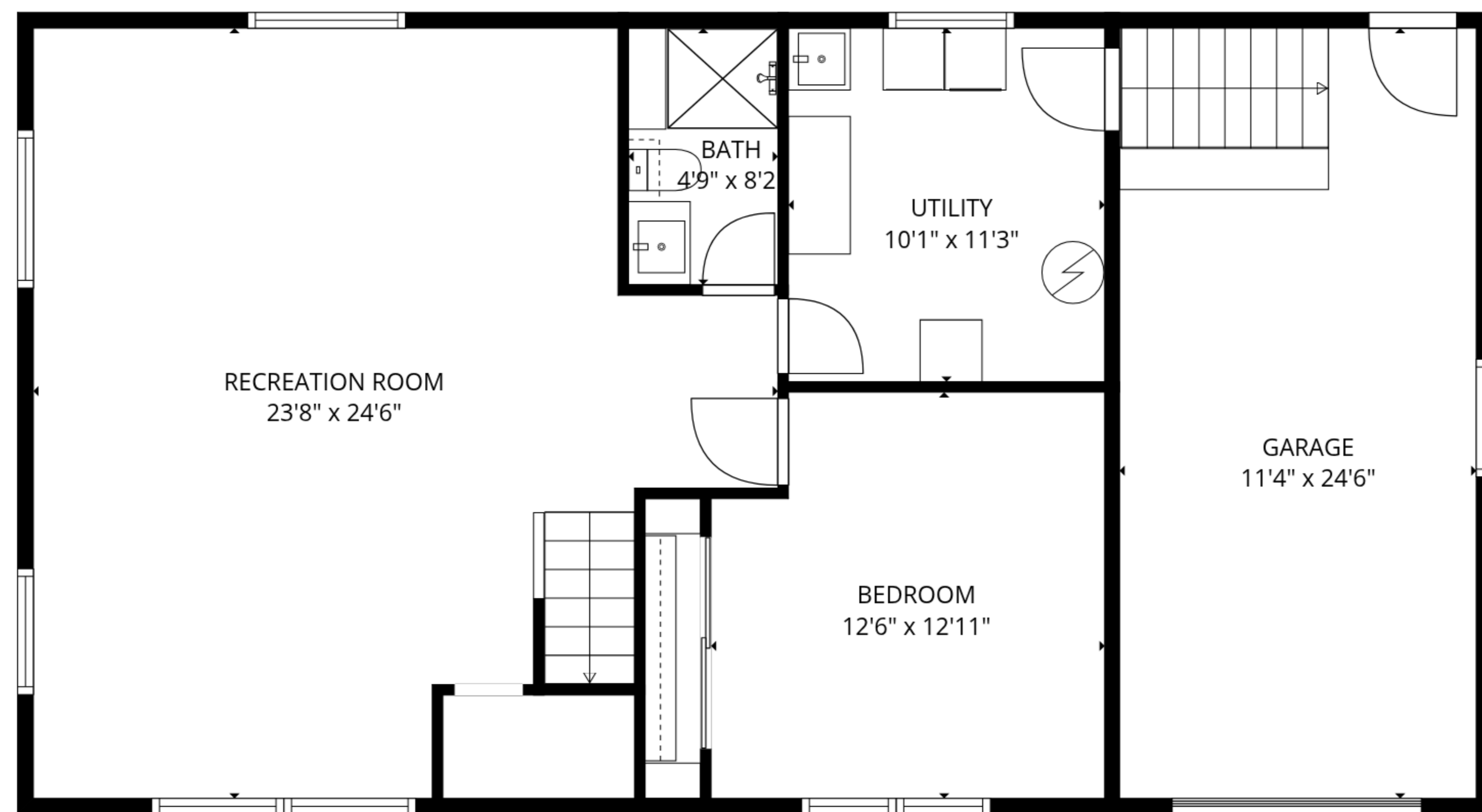
1st floor
