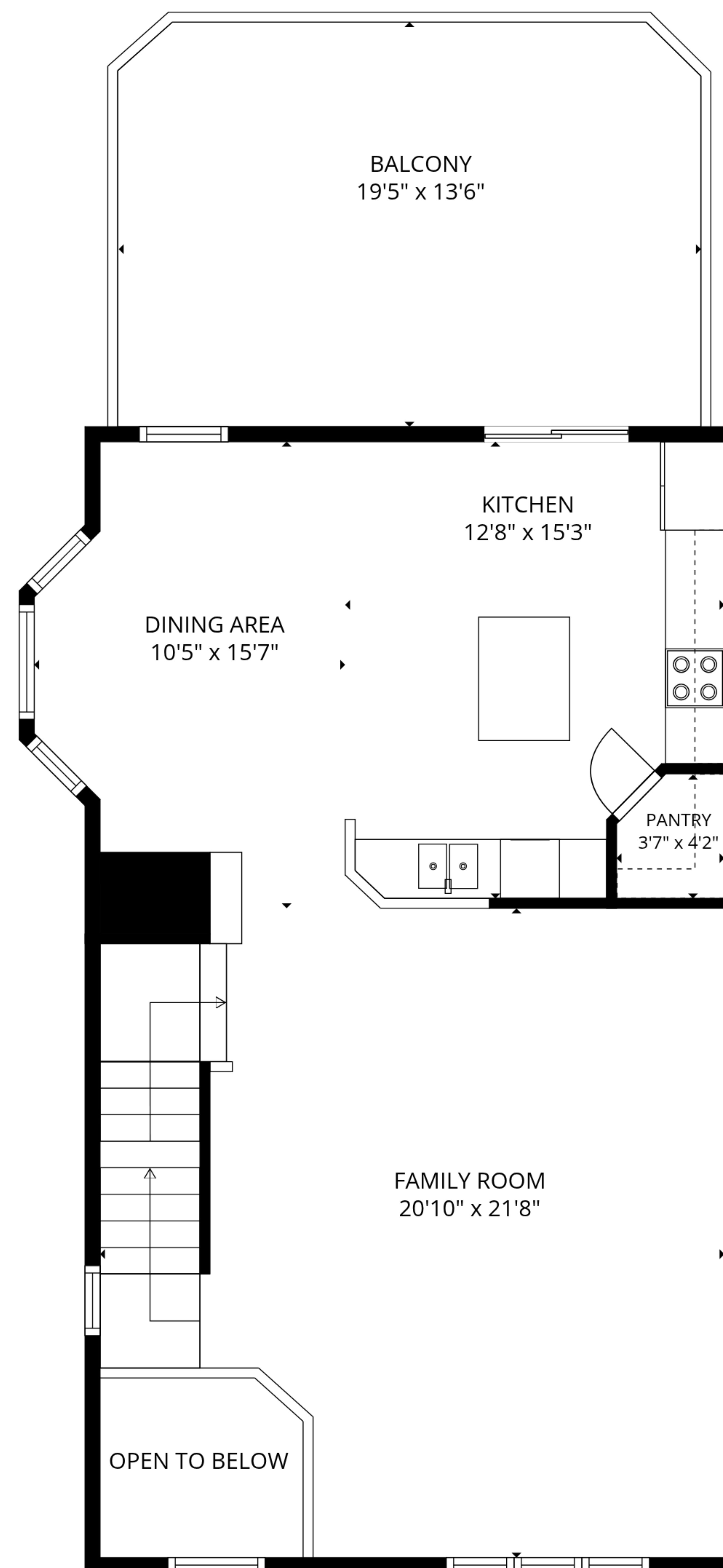
1st floor
