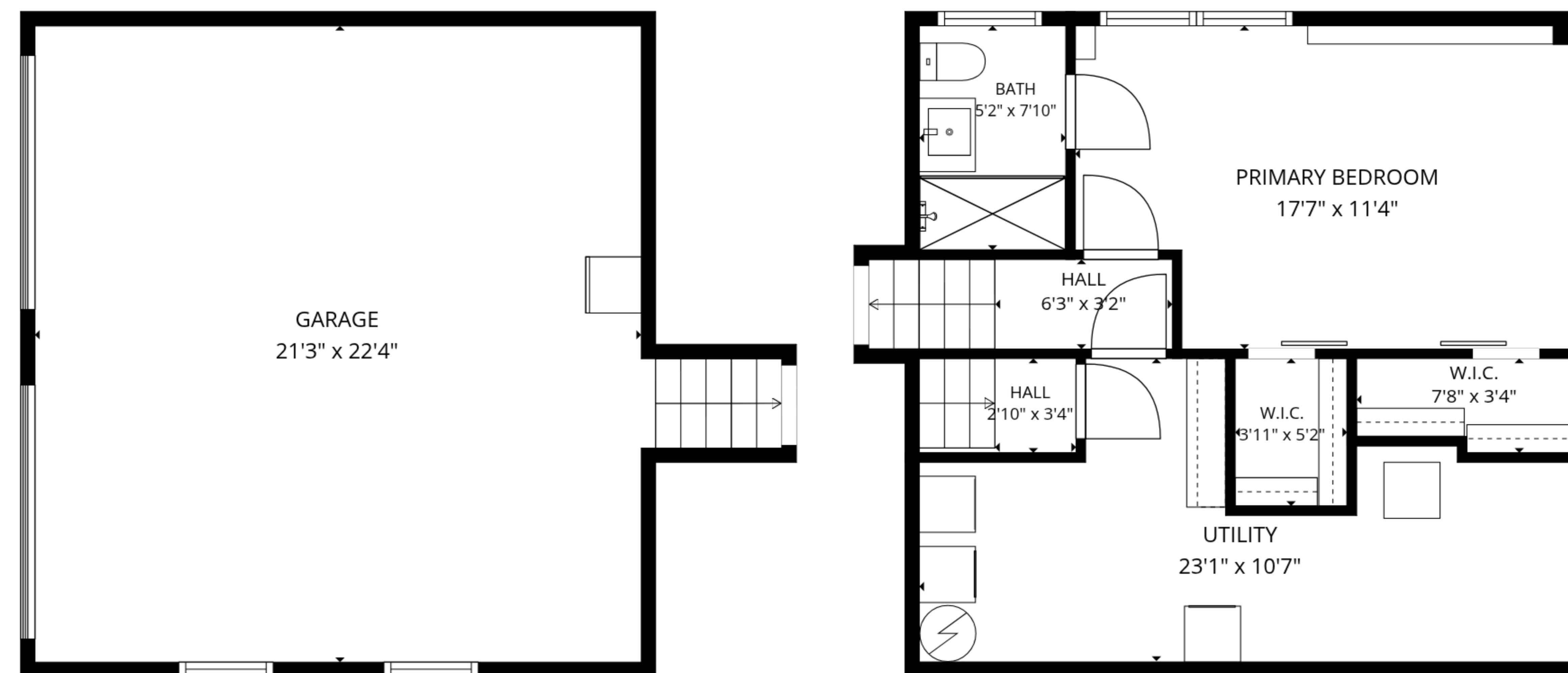
1st floor
