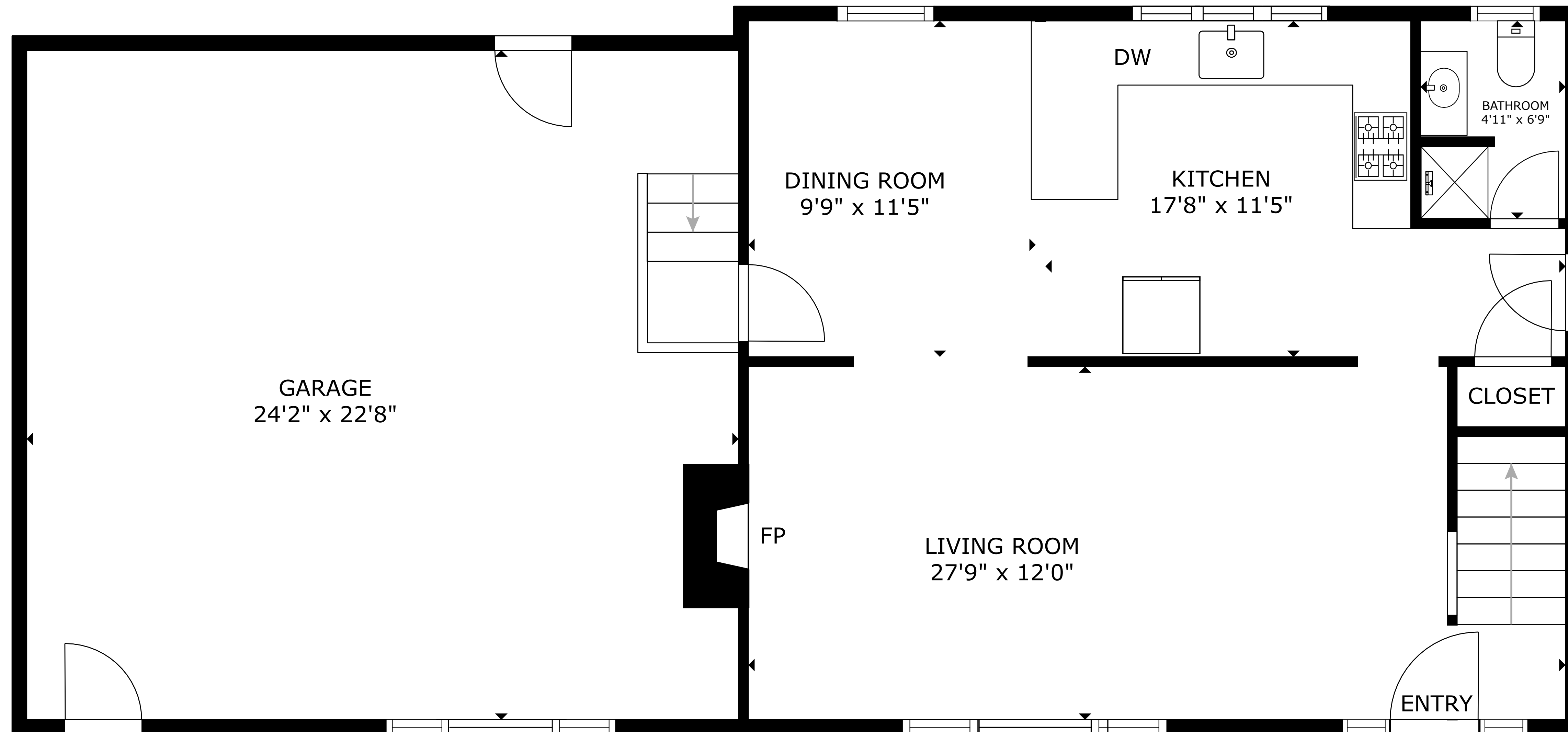
FLOOR 1
