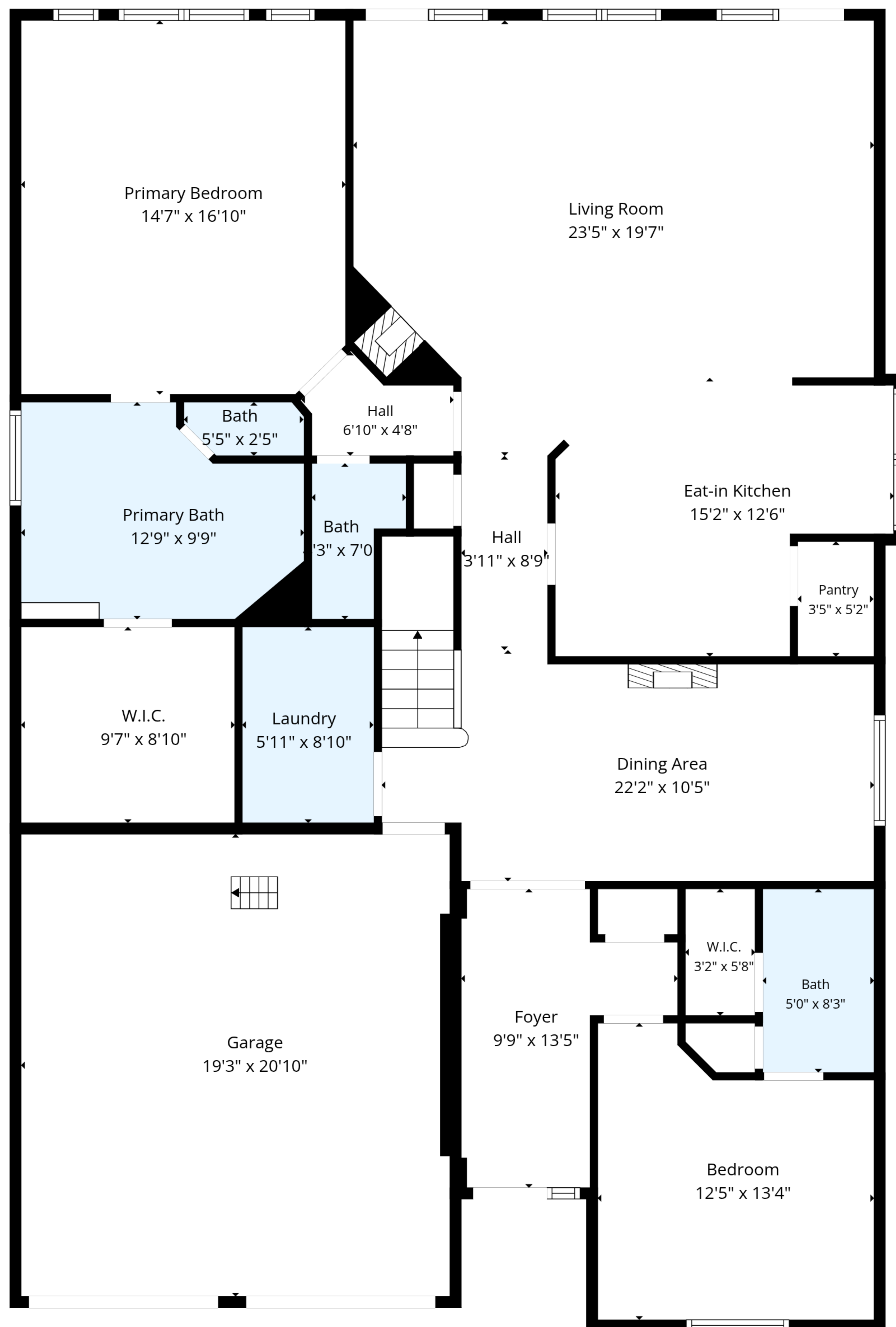
1st Floor
