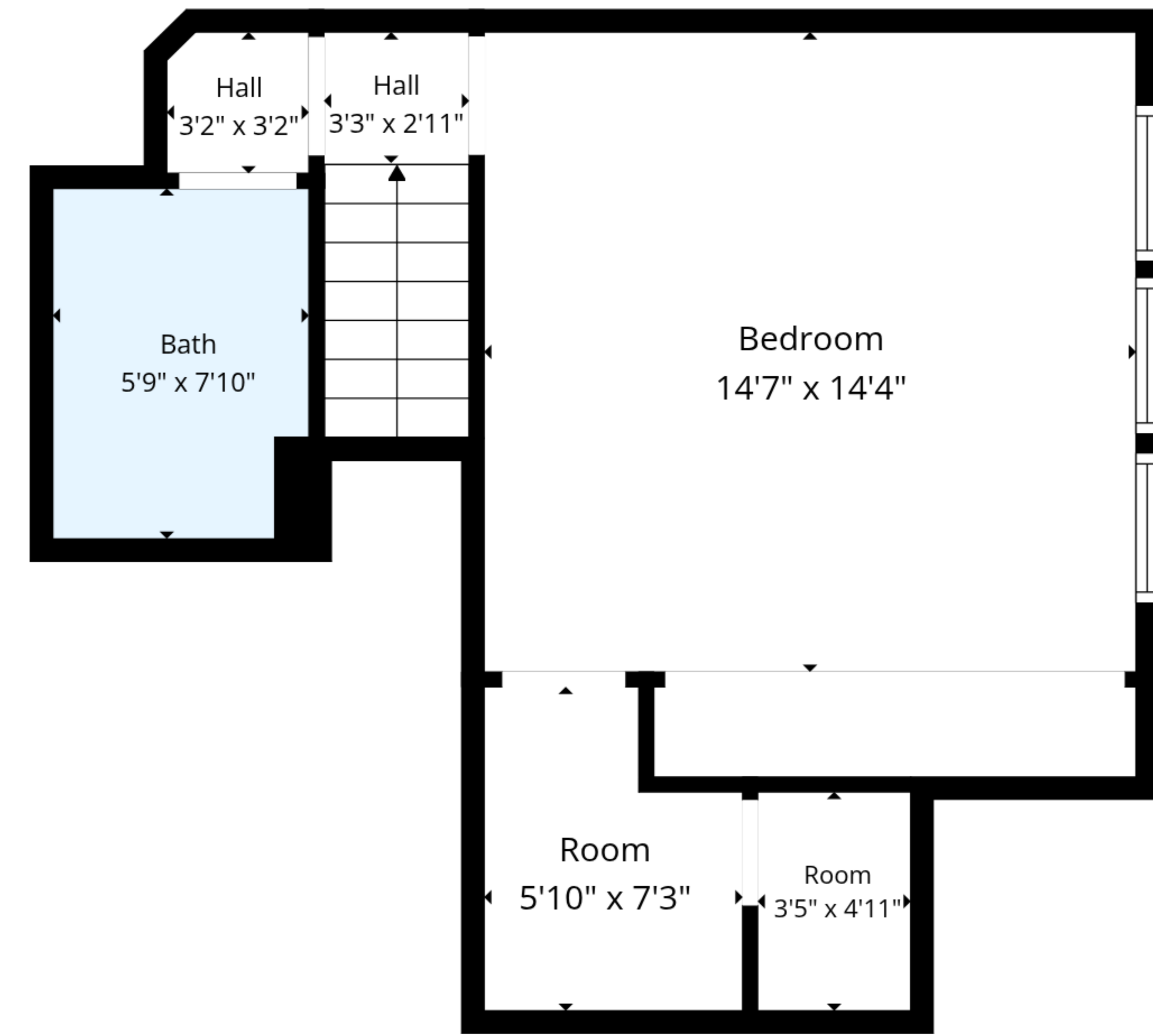
2nd Floor
