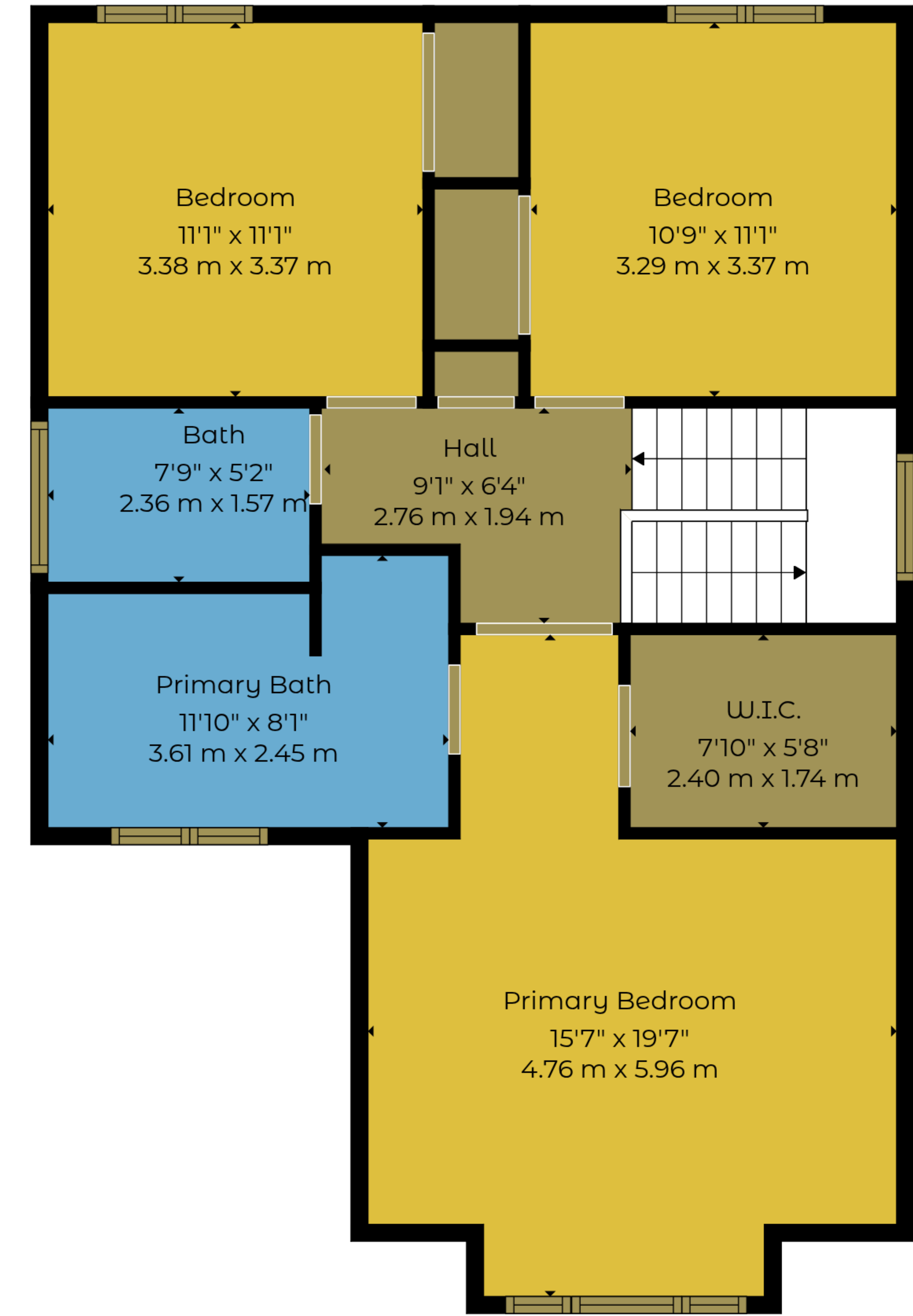
2nd Floor
