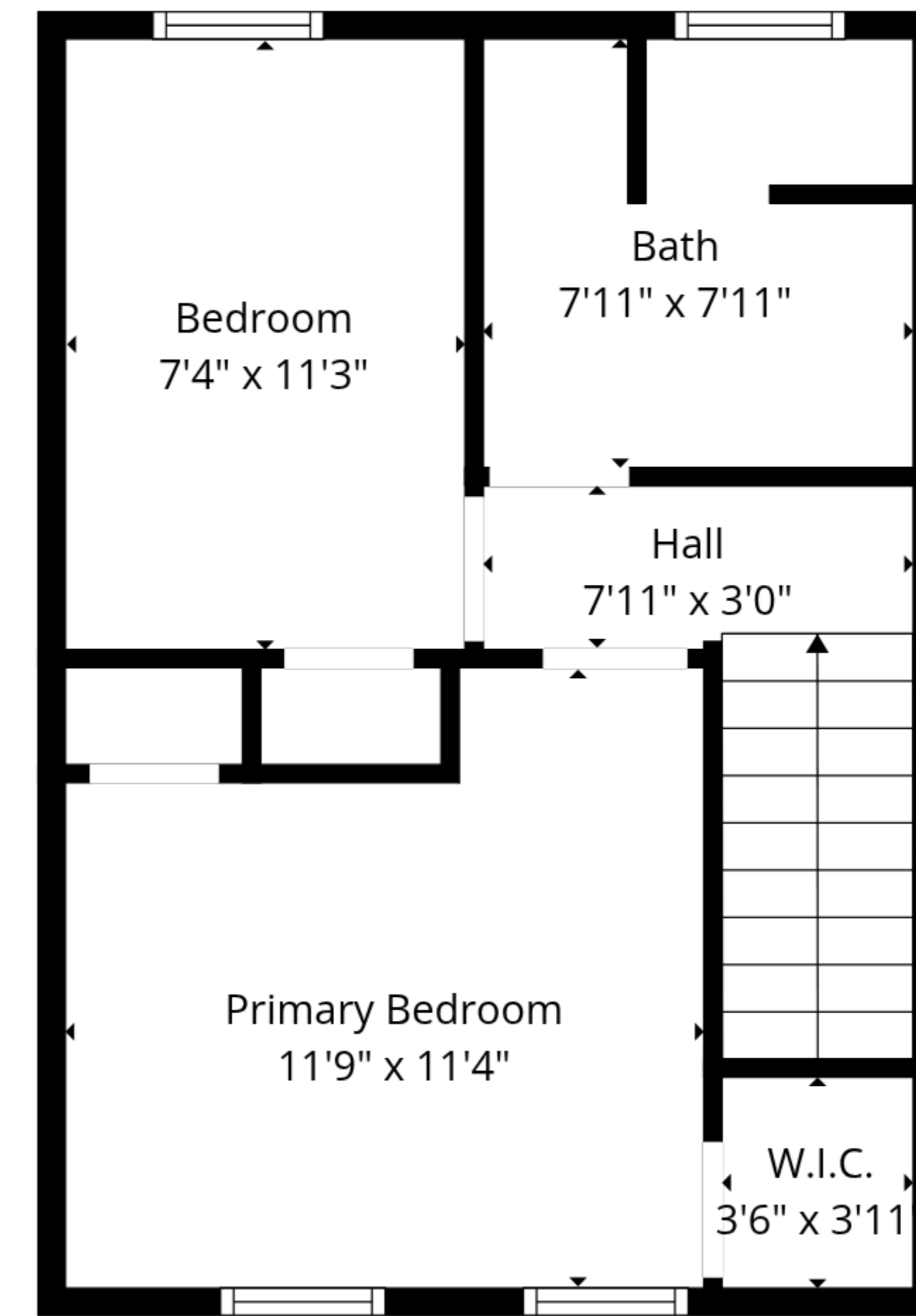
2nd Floor
