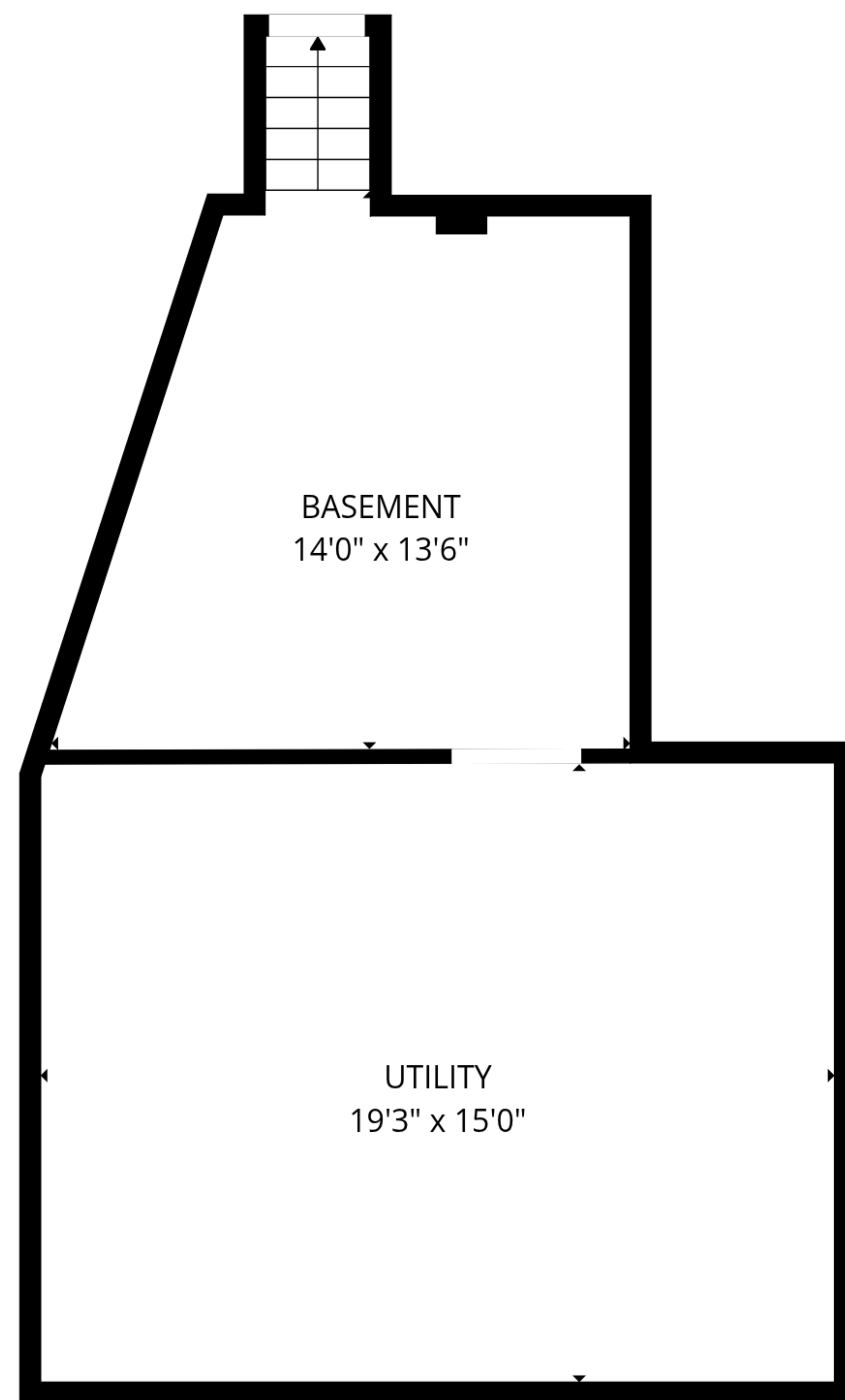
Basement 1
