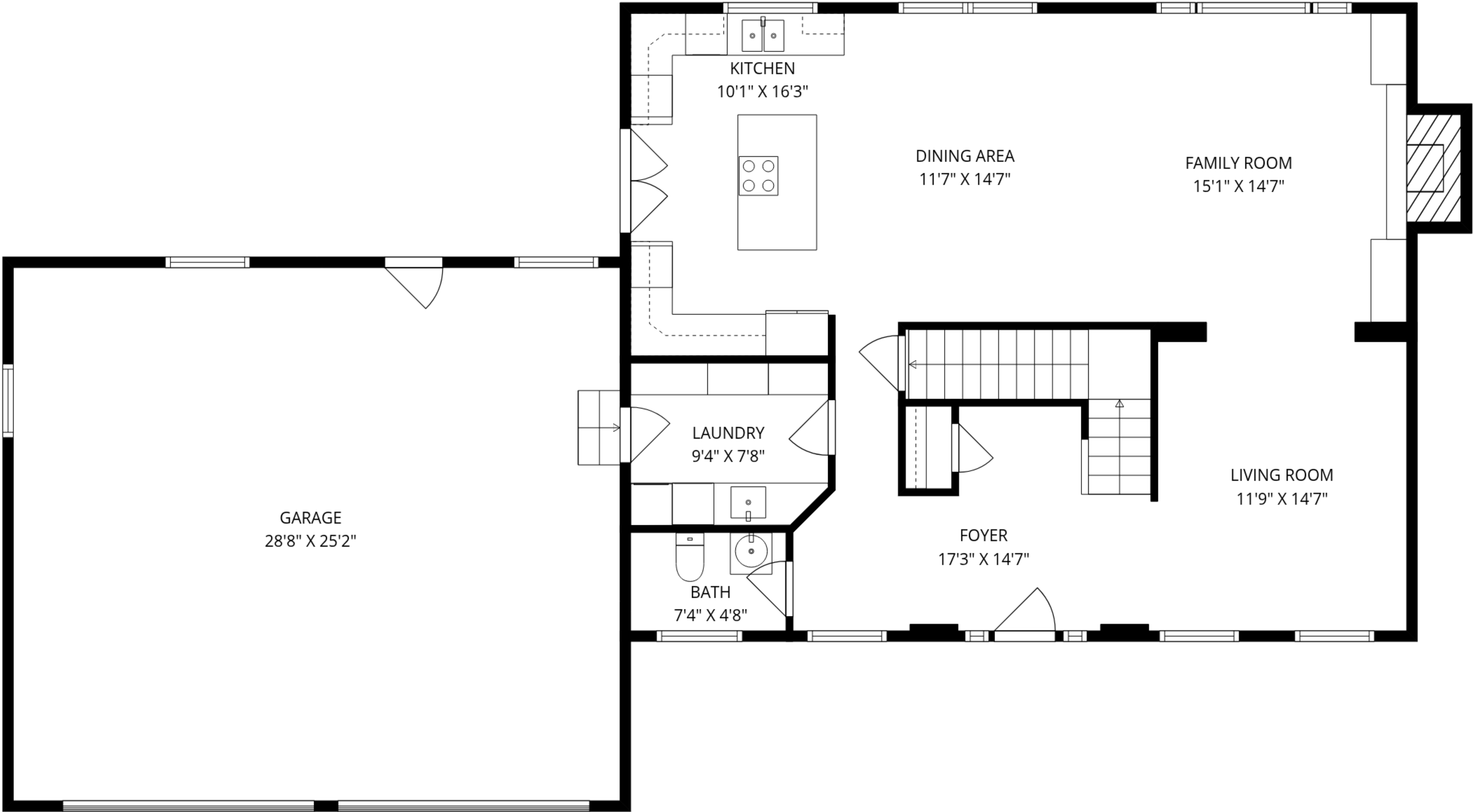
1ST FLOOR
