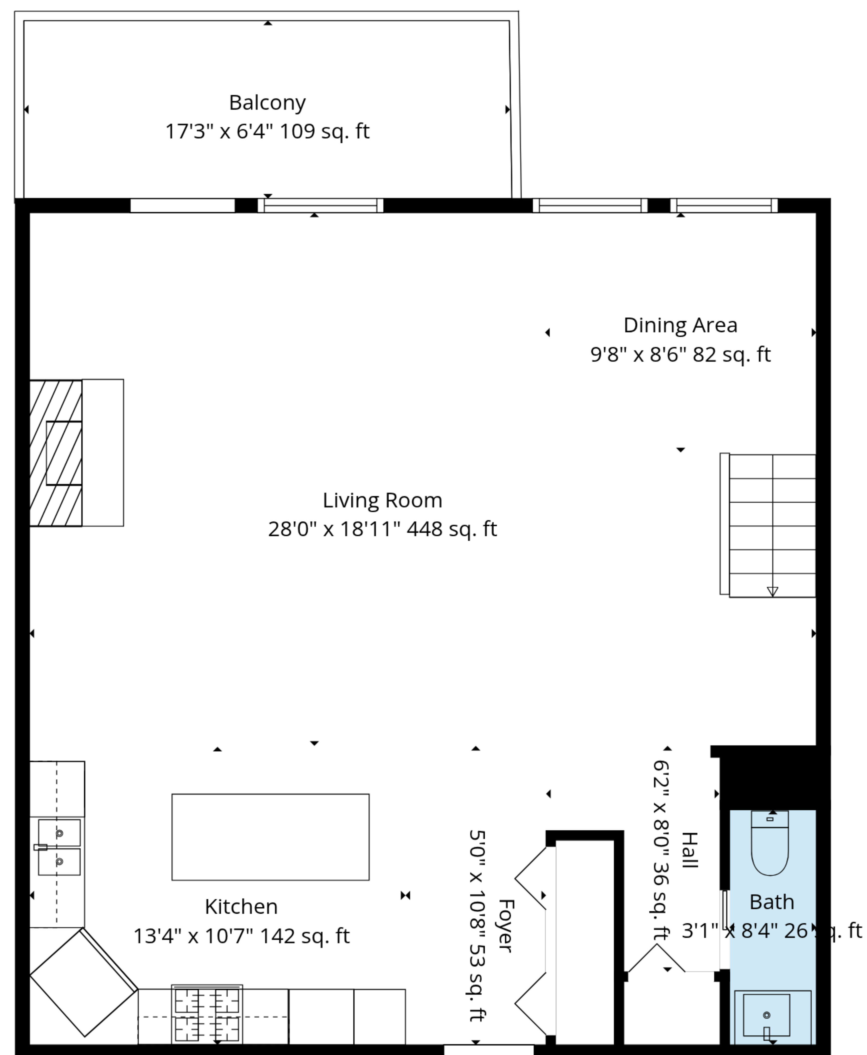
1st Floor
