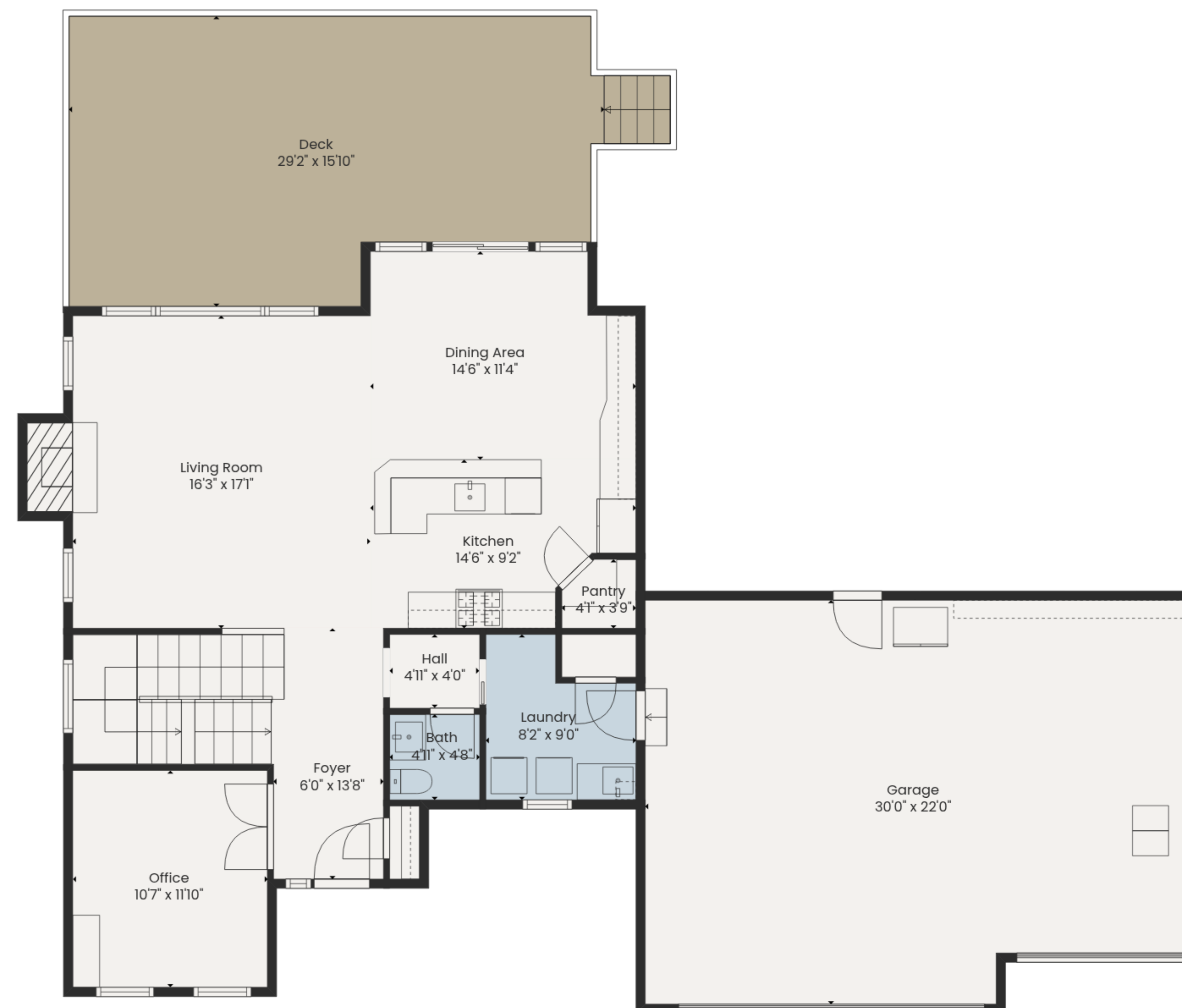
1st Floor
