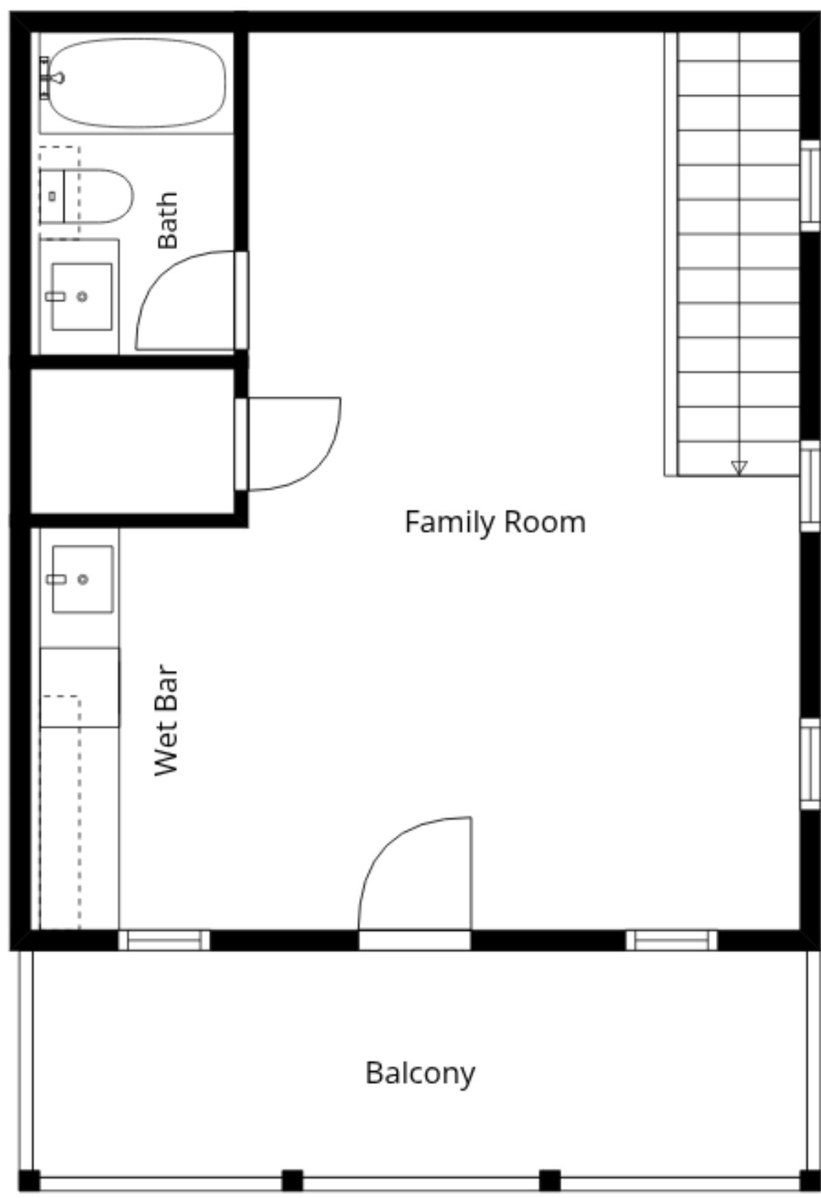
2nd Floor
