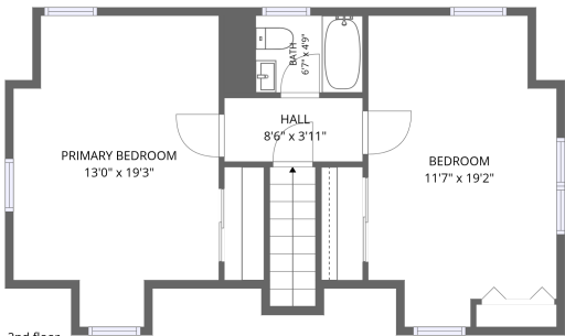
2nd floor
