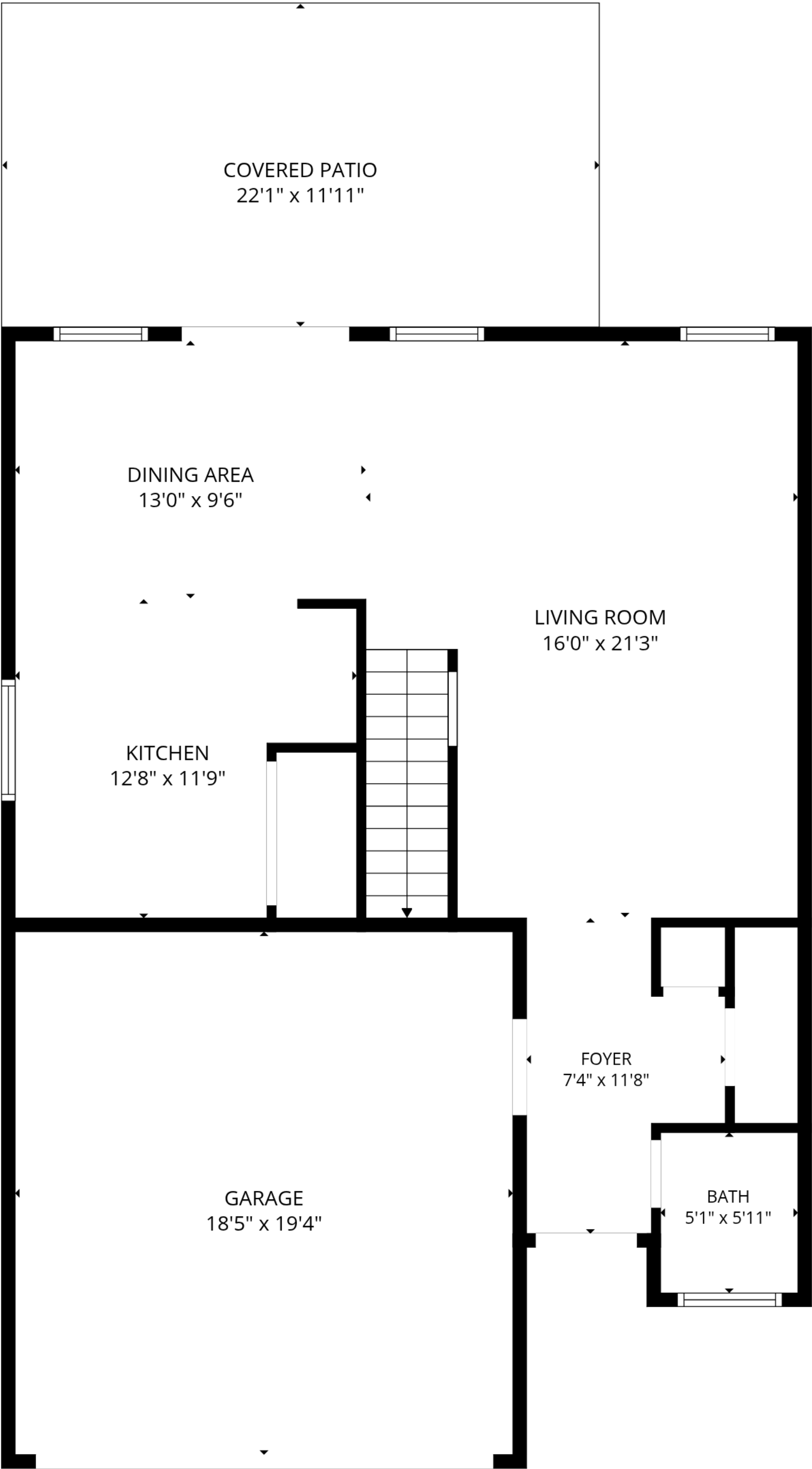
1st floor
