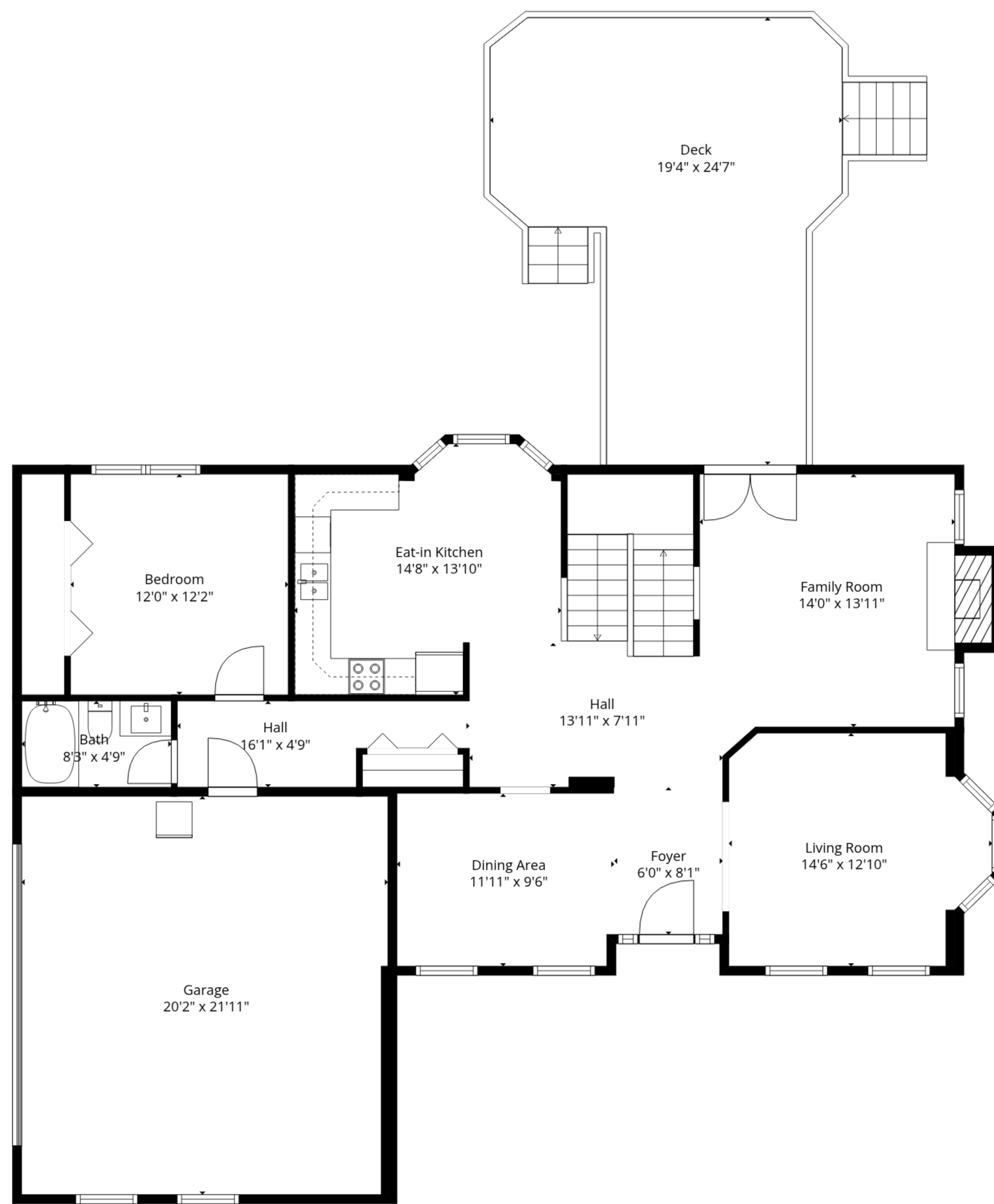
1st Floor
