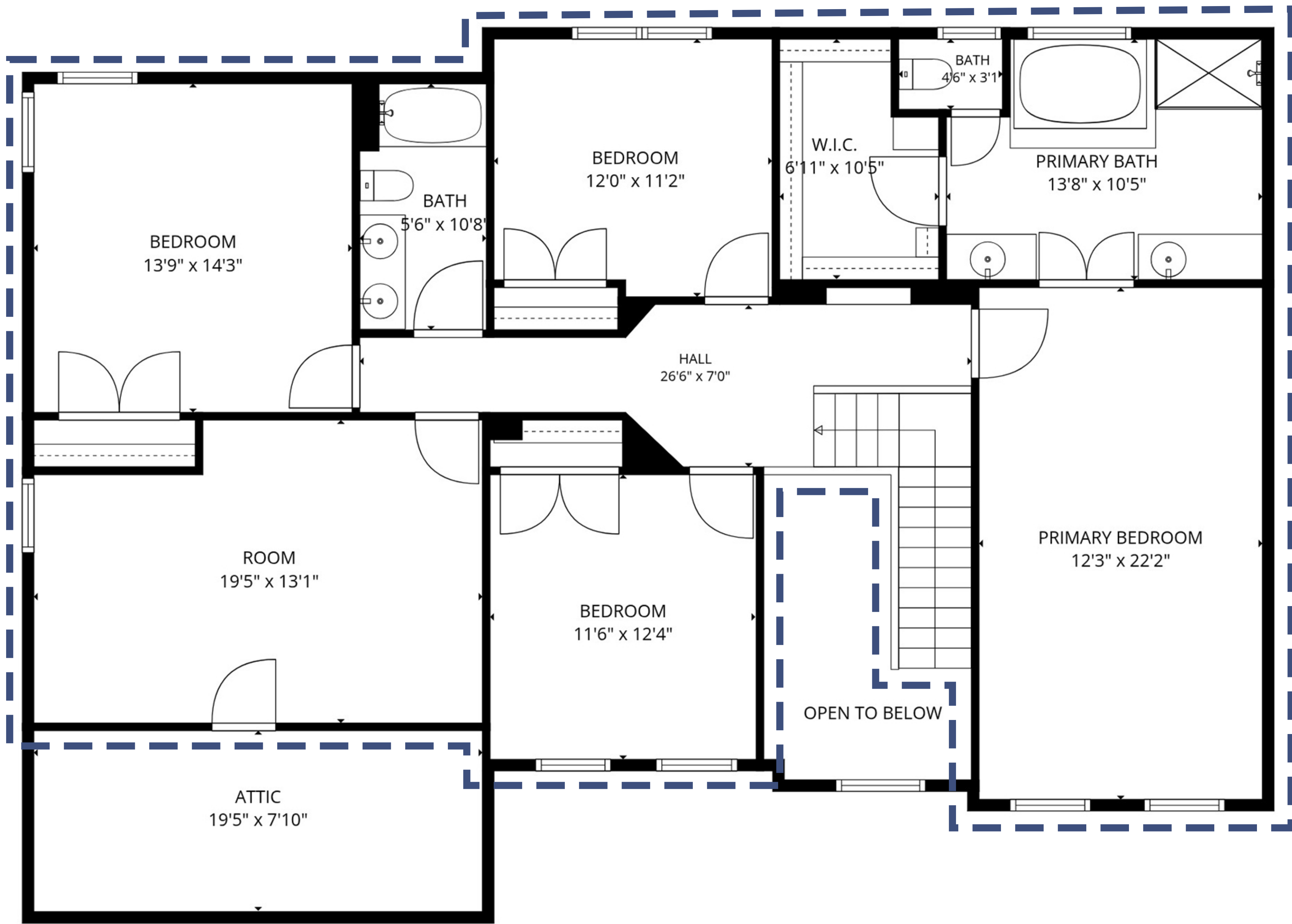
2nd floor
