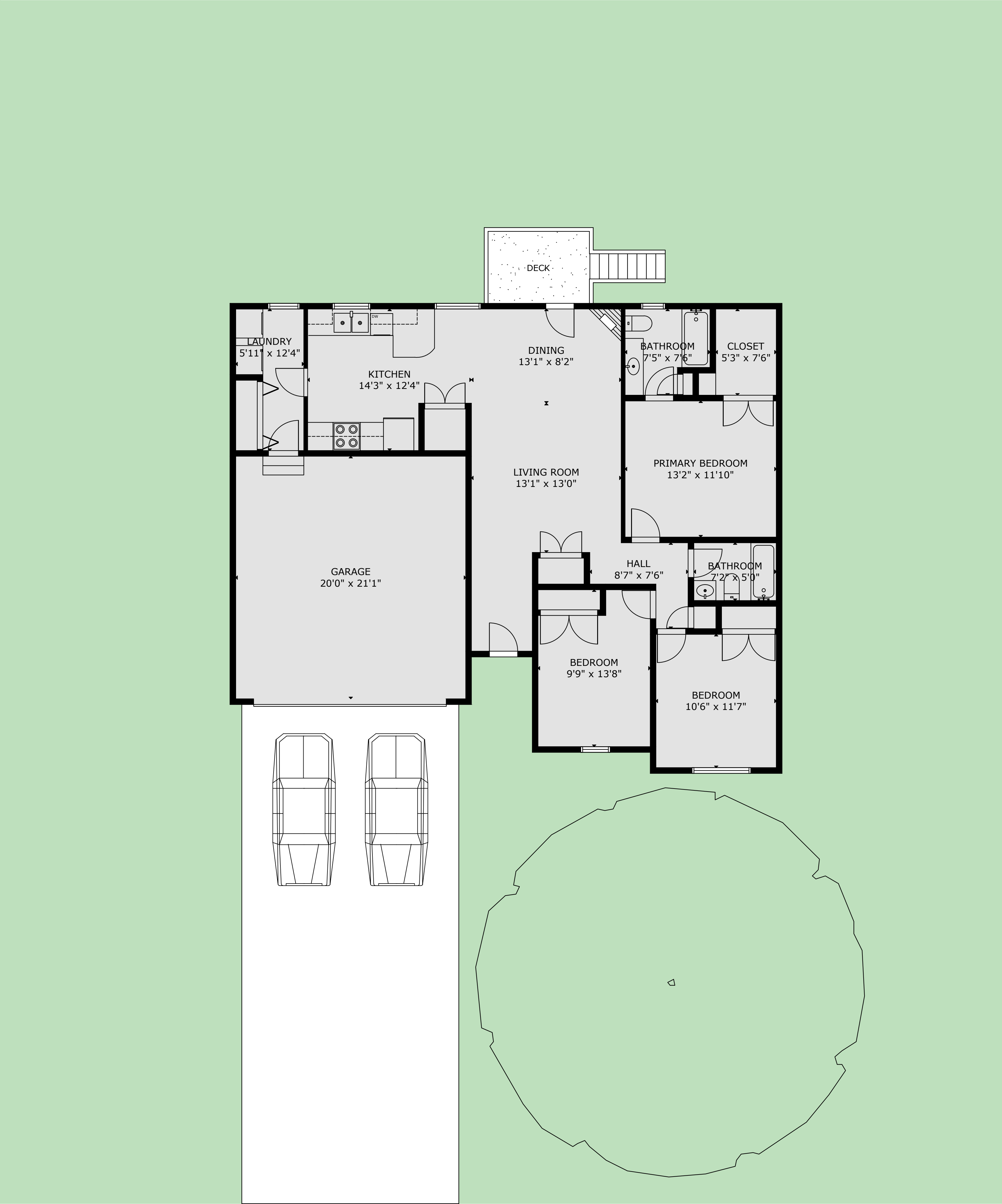
SITE PLAN
