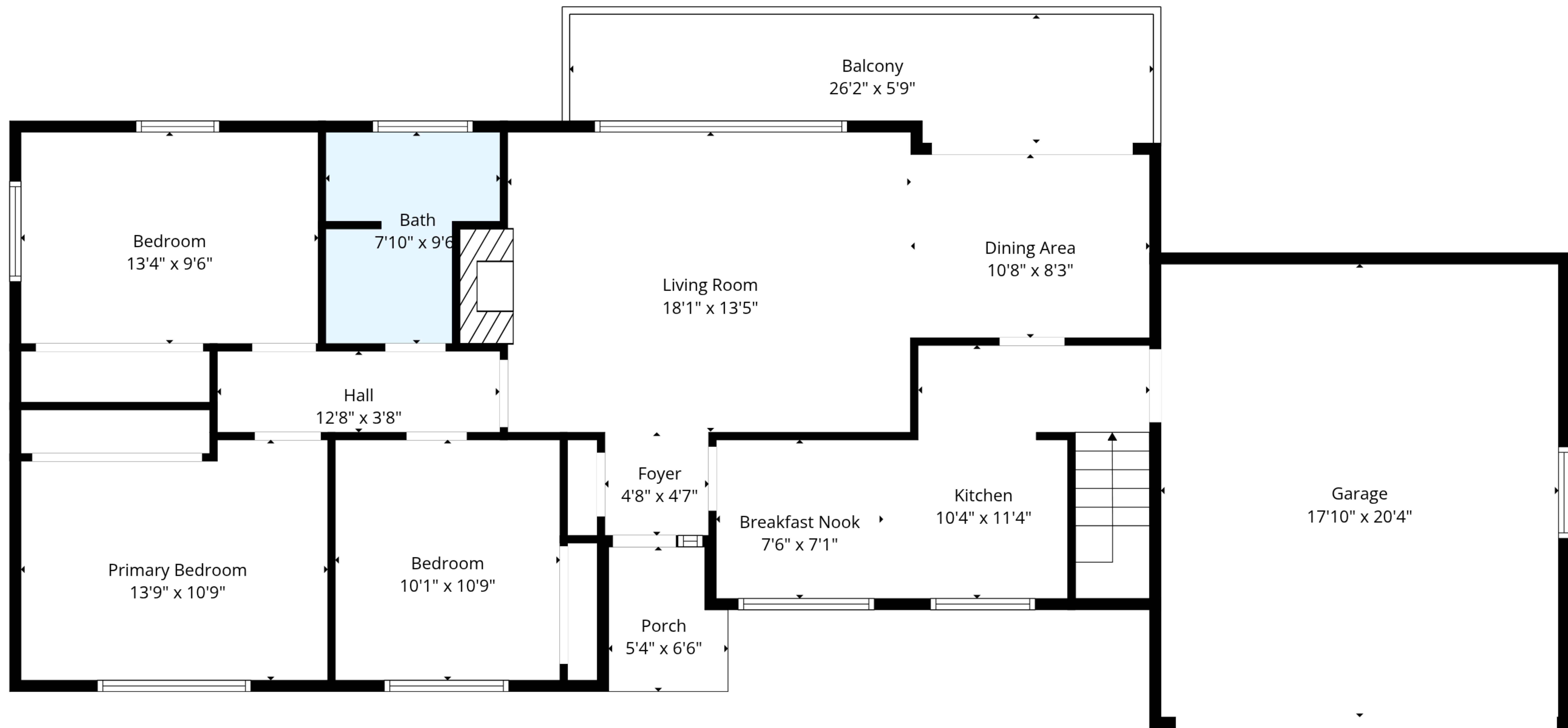
1st Floor
