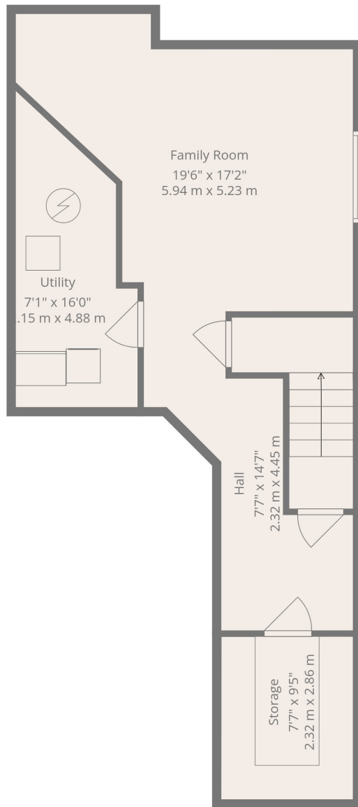
Basement
