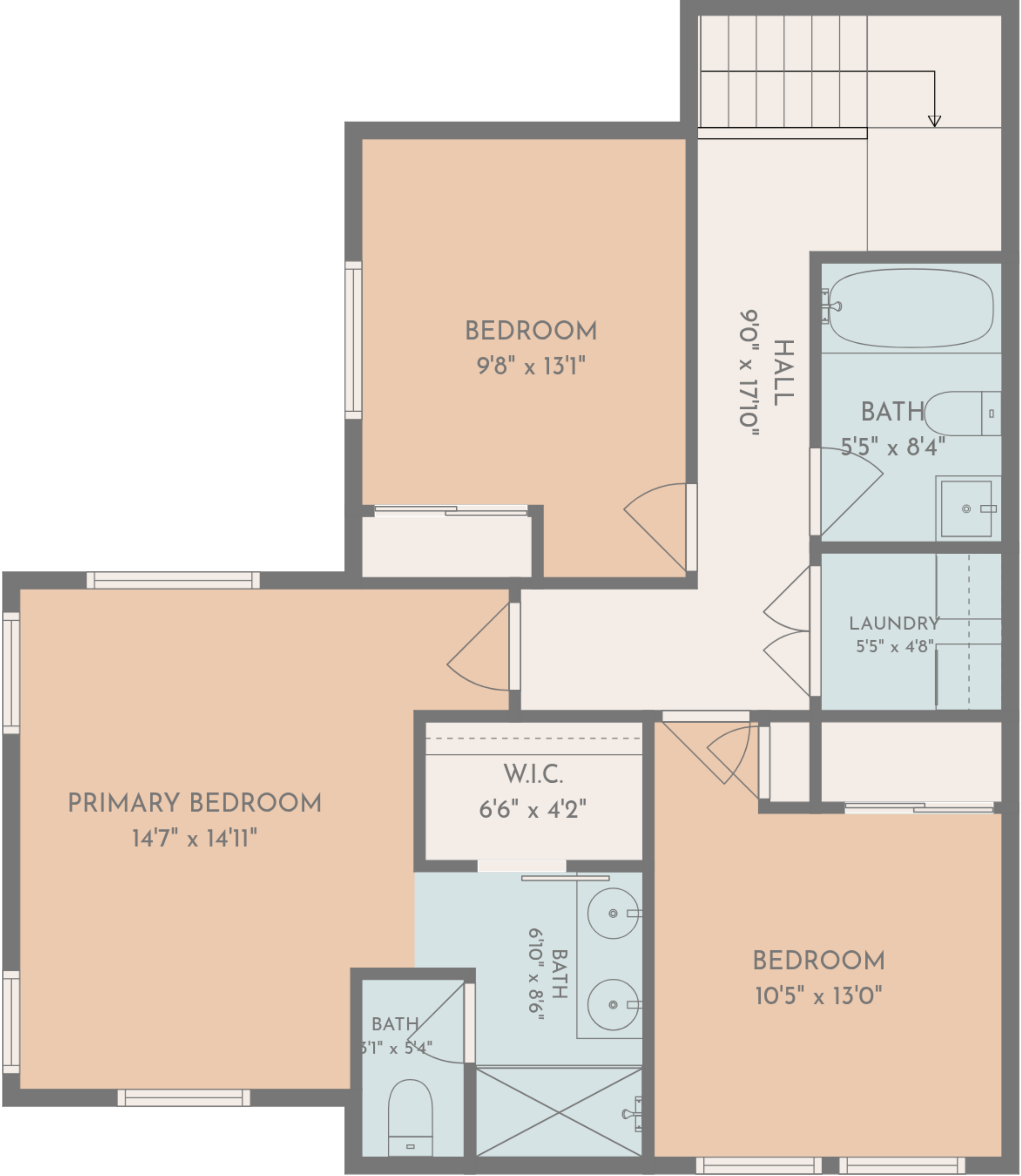
2nd floor
