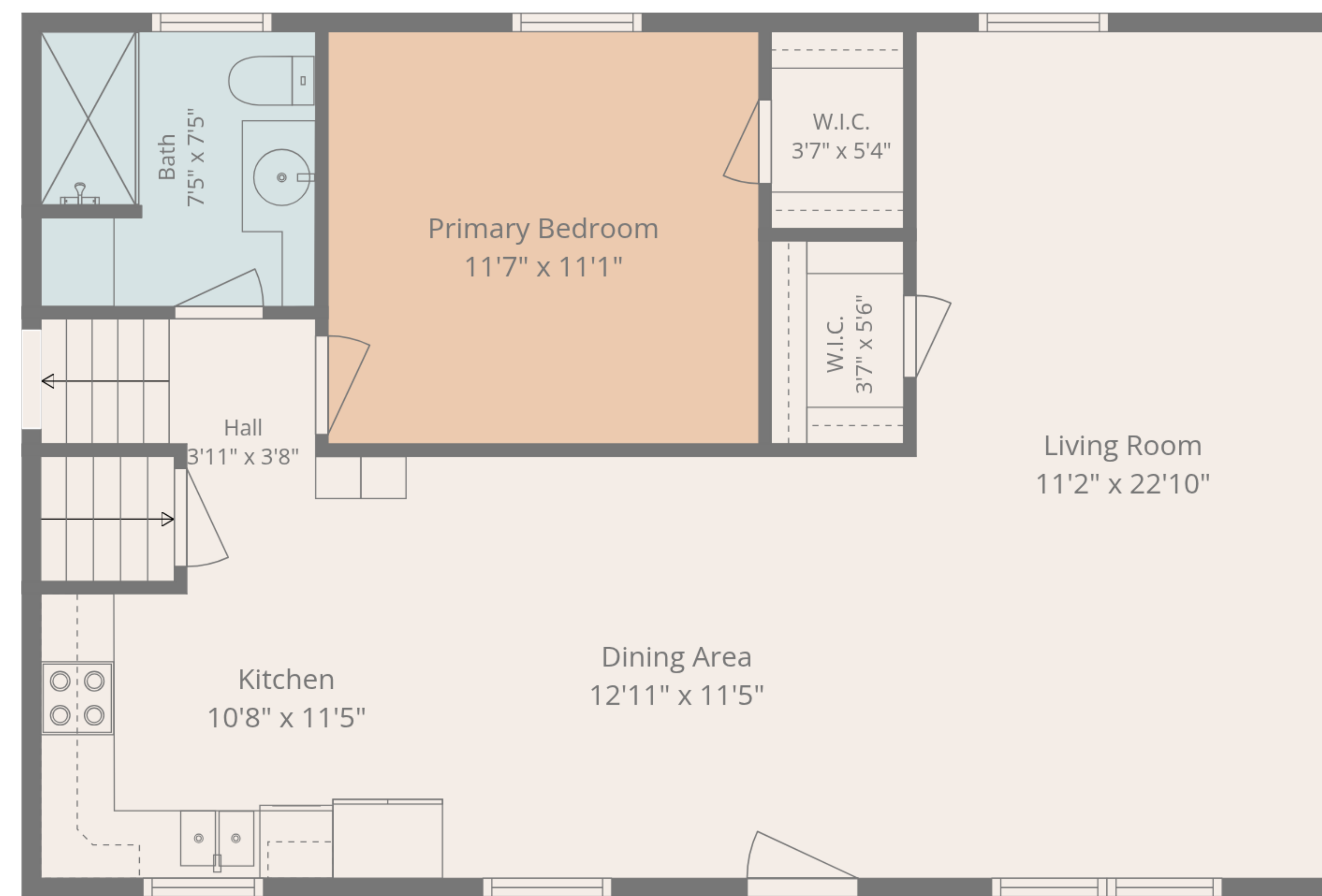
3rd Floor
