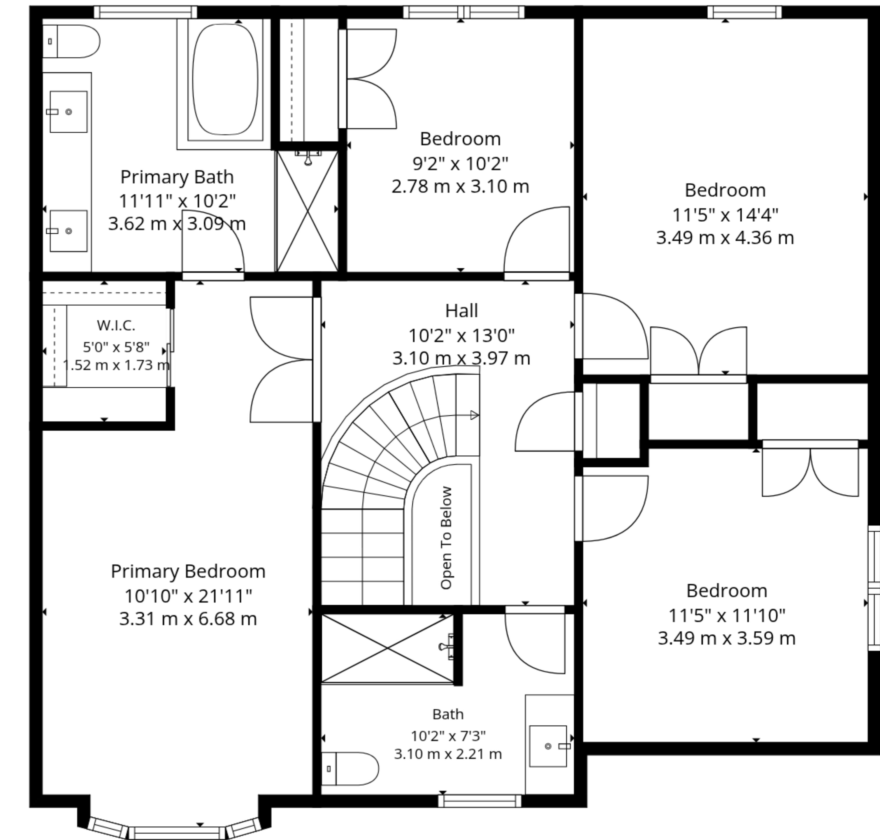
2nd Floor
