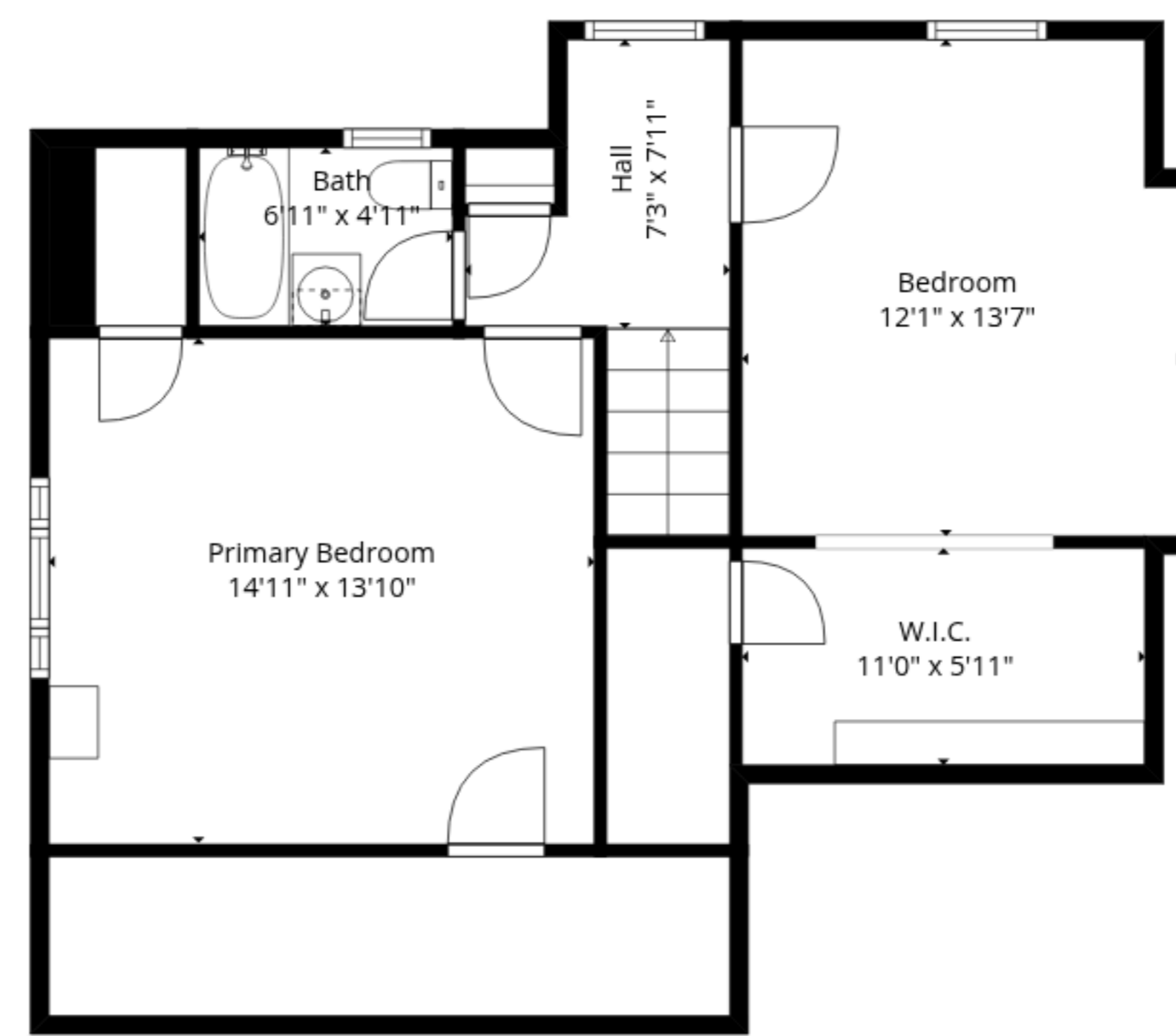
3rd Floor
