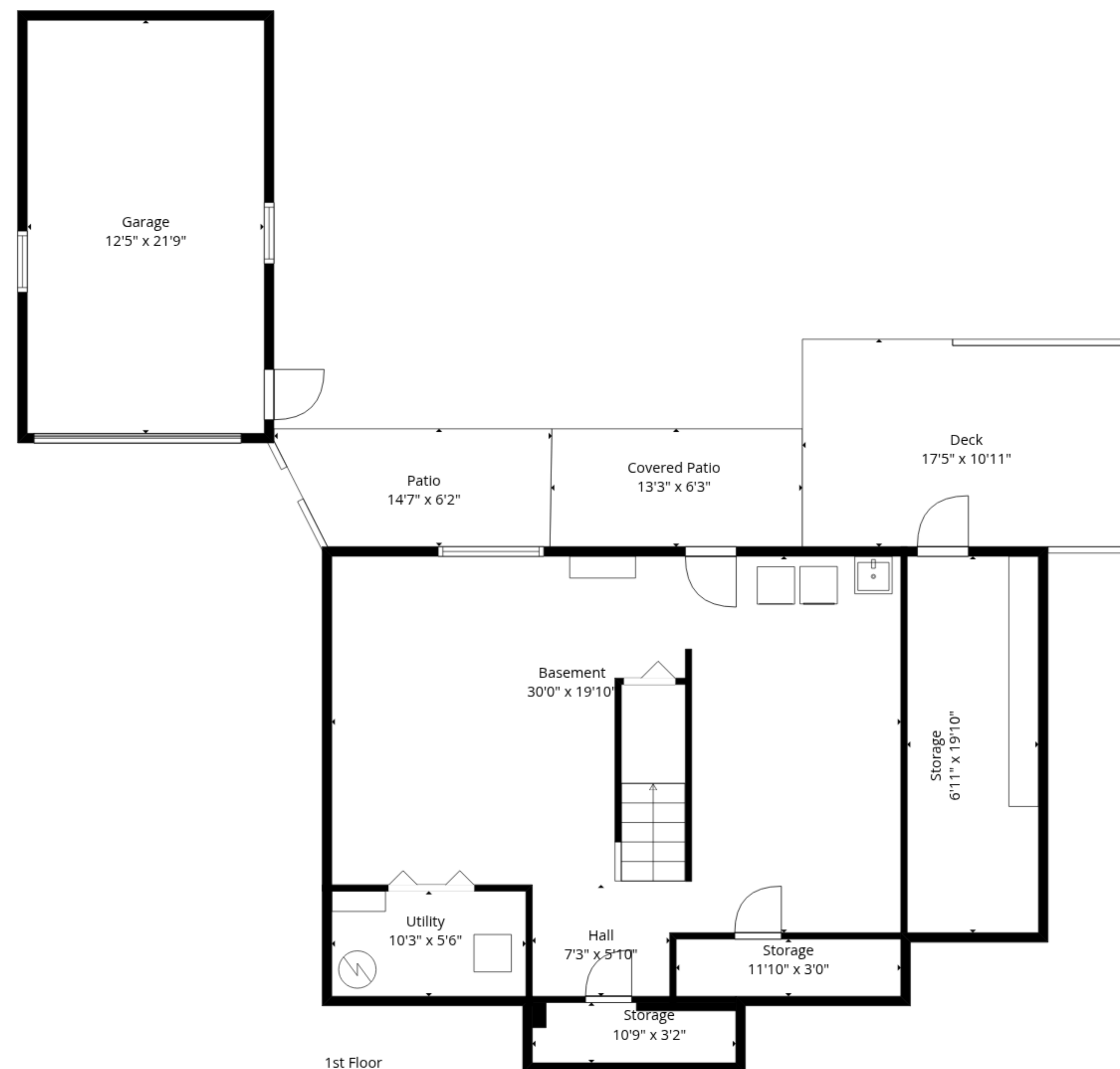
1st Floor
