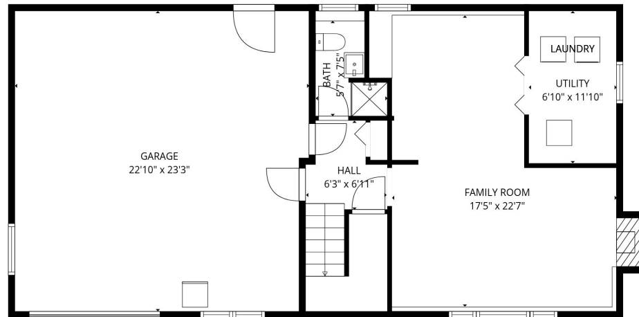
1st floor
