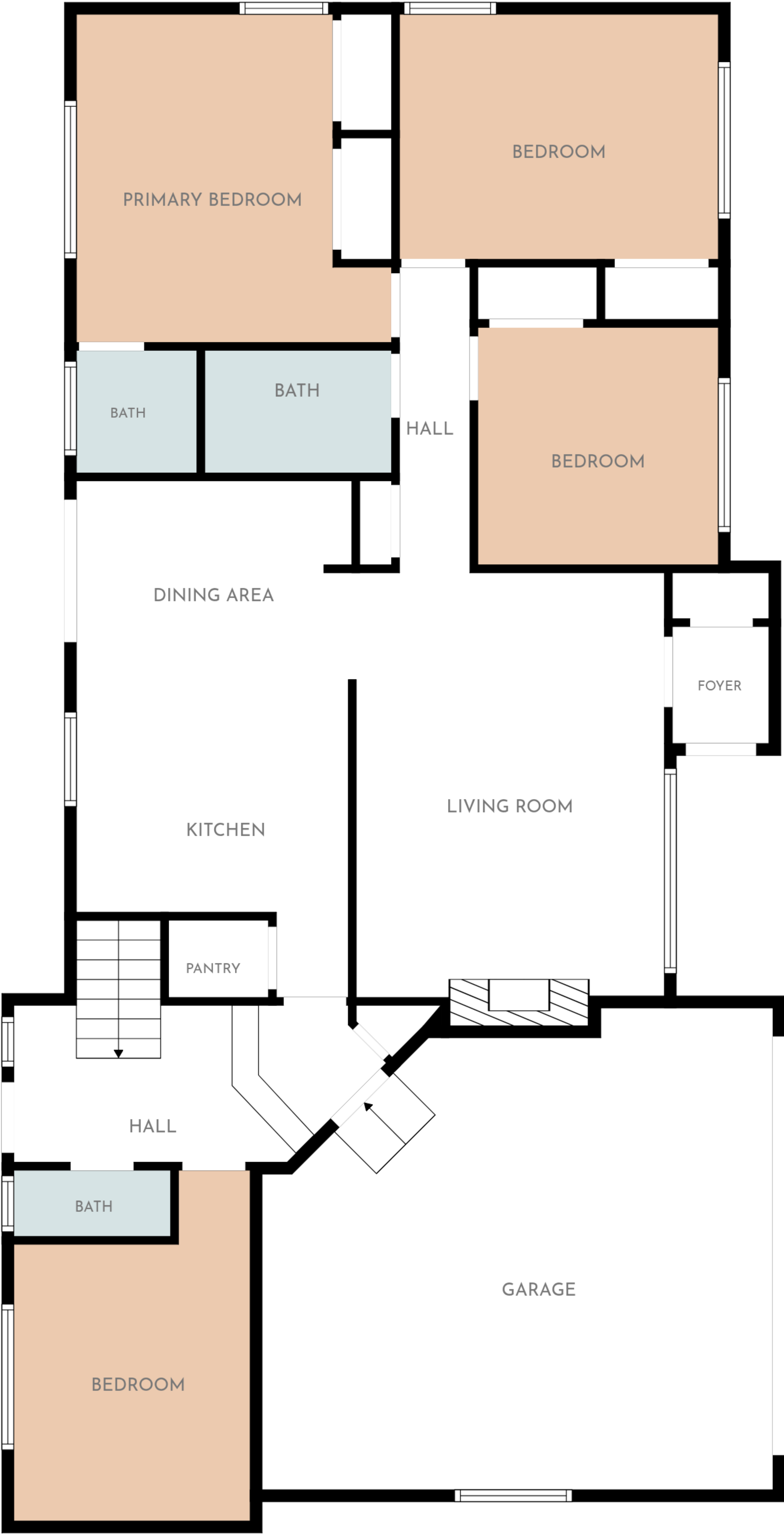
1st floor
